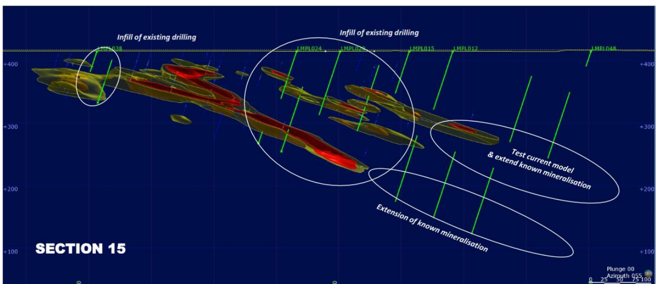
Figure 4: Lady Magdalene cross section 15 looking north-east showing CLZ proposed drill holes
