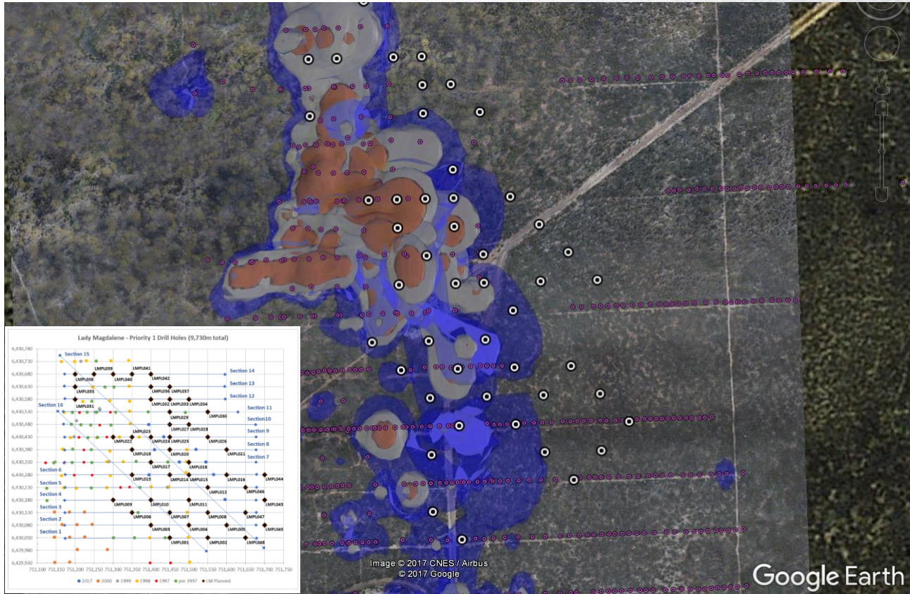
Figure 3: Planned Holes (white) at Lady Magdalene Plotted Against Previous Drill Collars (pink) and the latest implicit model
