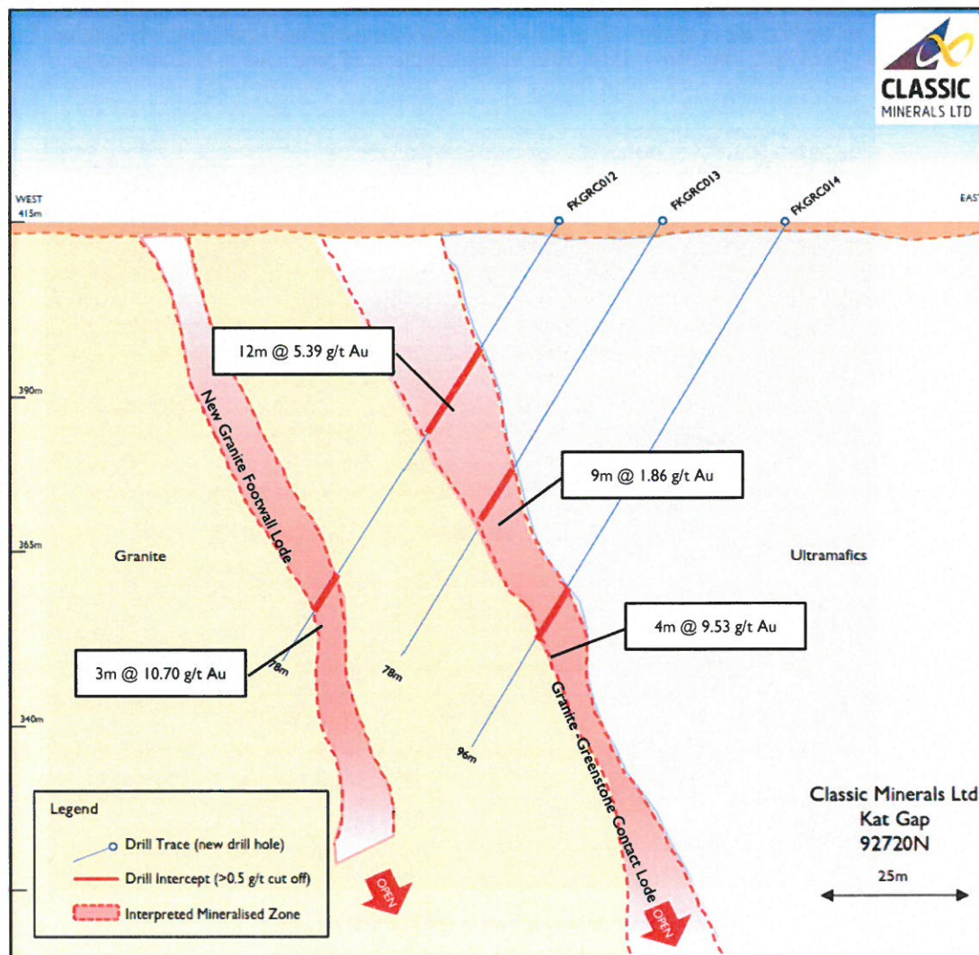
Figure 2: Kat Gap Cross Section 92720 (local grid) Looking North
