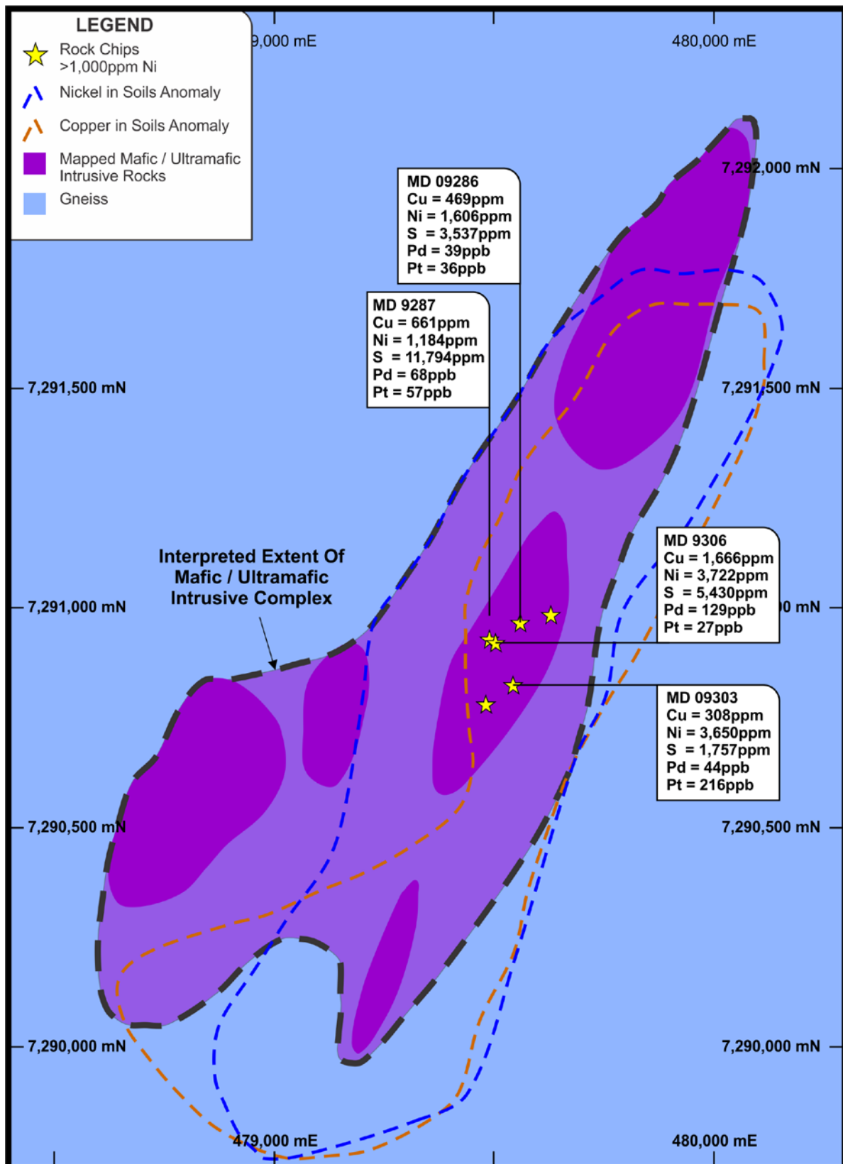
Figure (3) – Target C: Schematic Geology and Rock Chip Results
