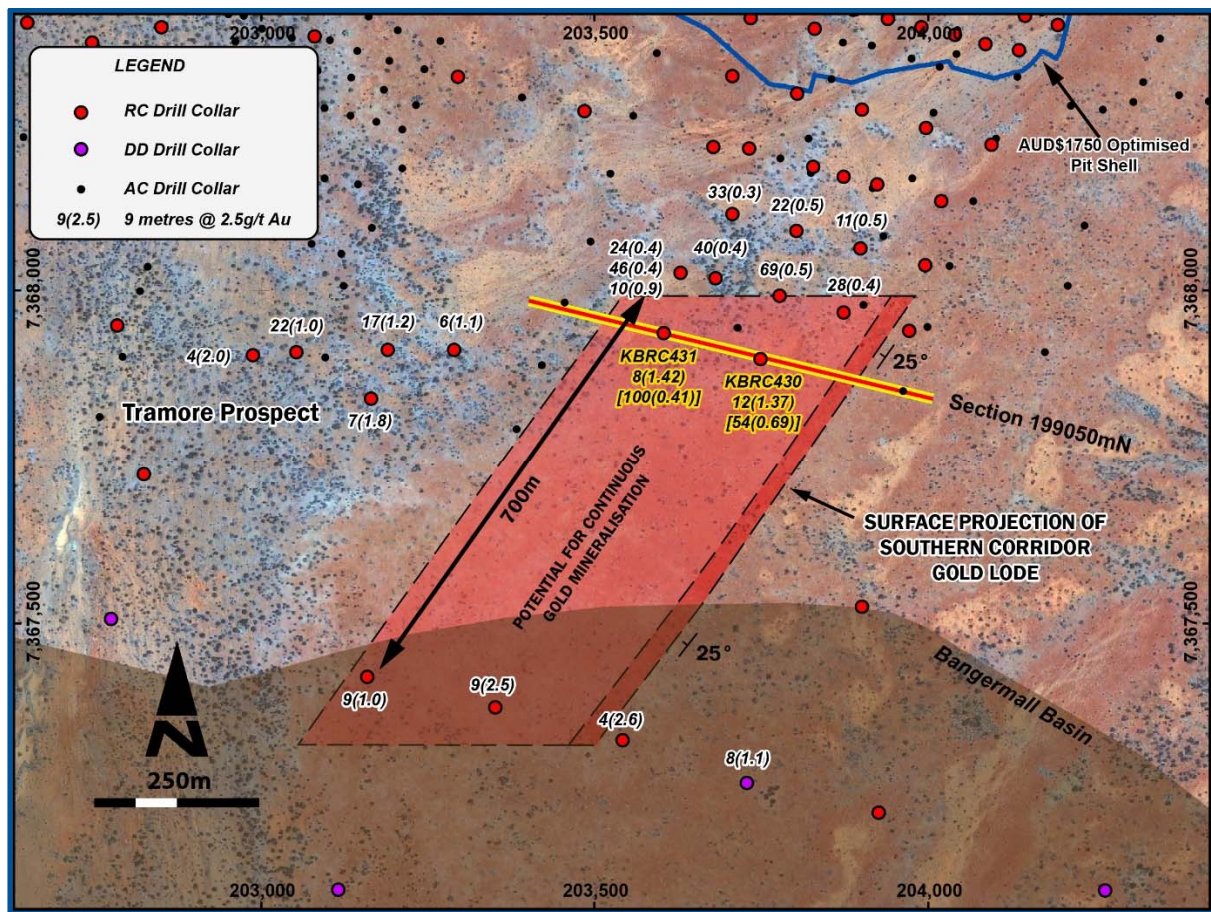
Figure 4: Southern Corridor Prospect Drilling Results (Plan)
