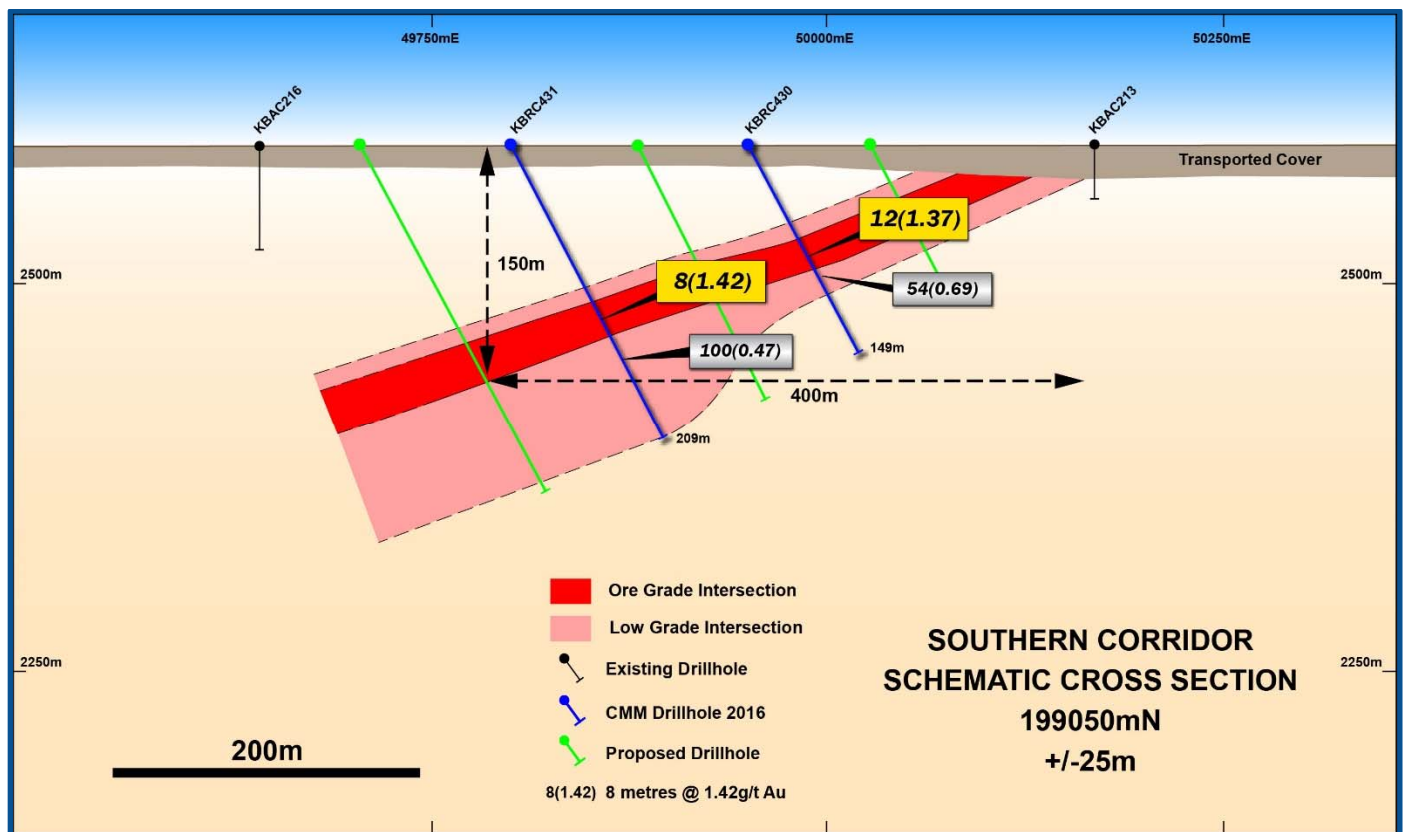
Figure 3: Southern Corridor Drilling Results (Section 199900mN)
