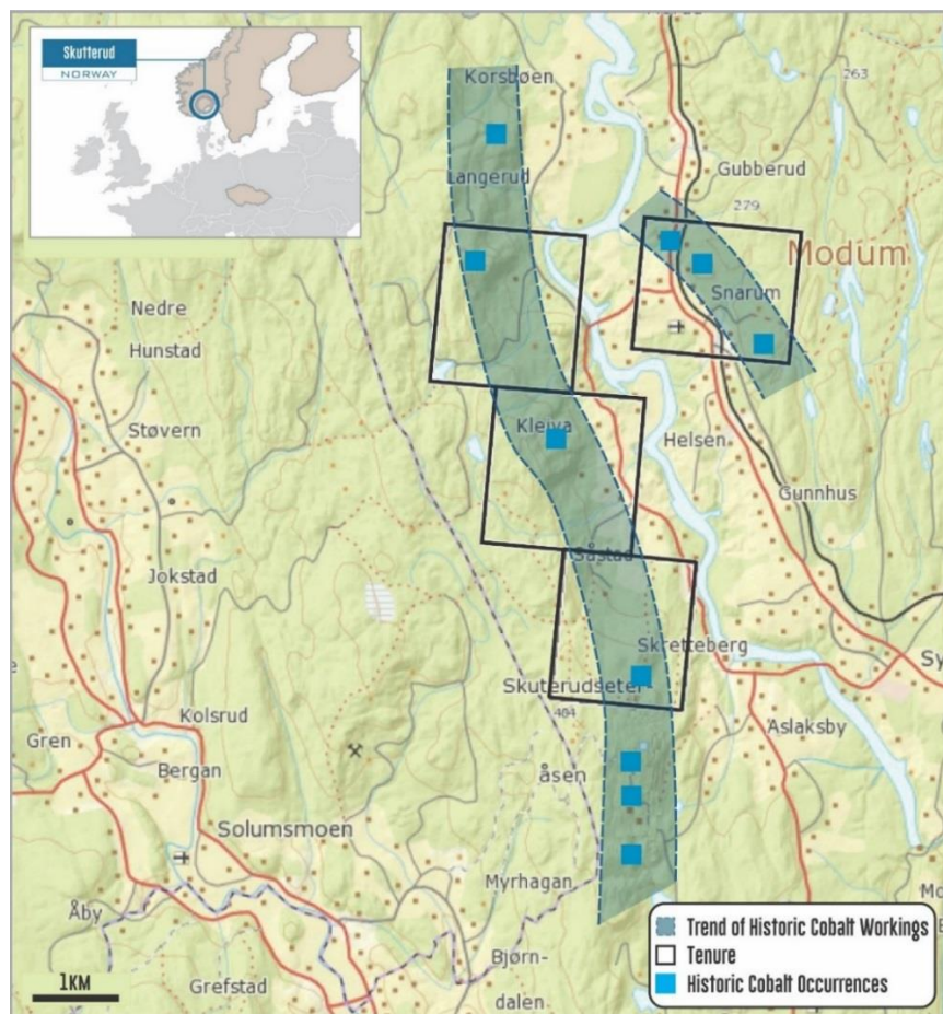
Figure 3 | Skutterud Project area and historic cobalt occurrences
