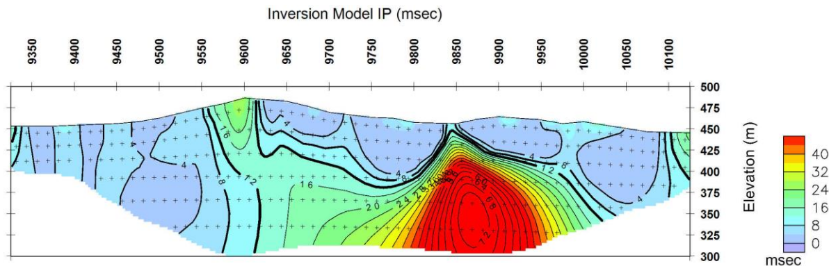
Figure 2. IP Line 20320N Inversion showing strong chargeability at the GAP Target
