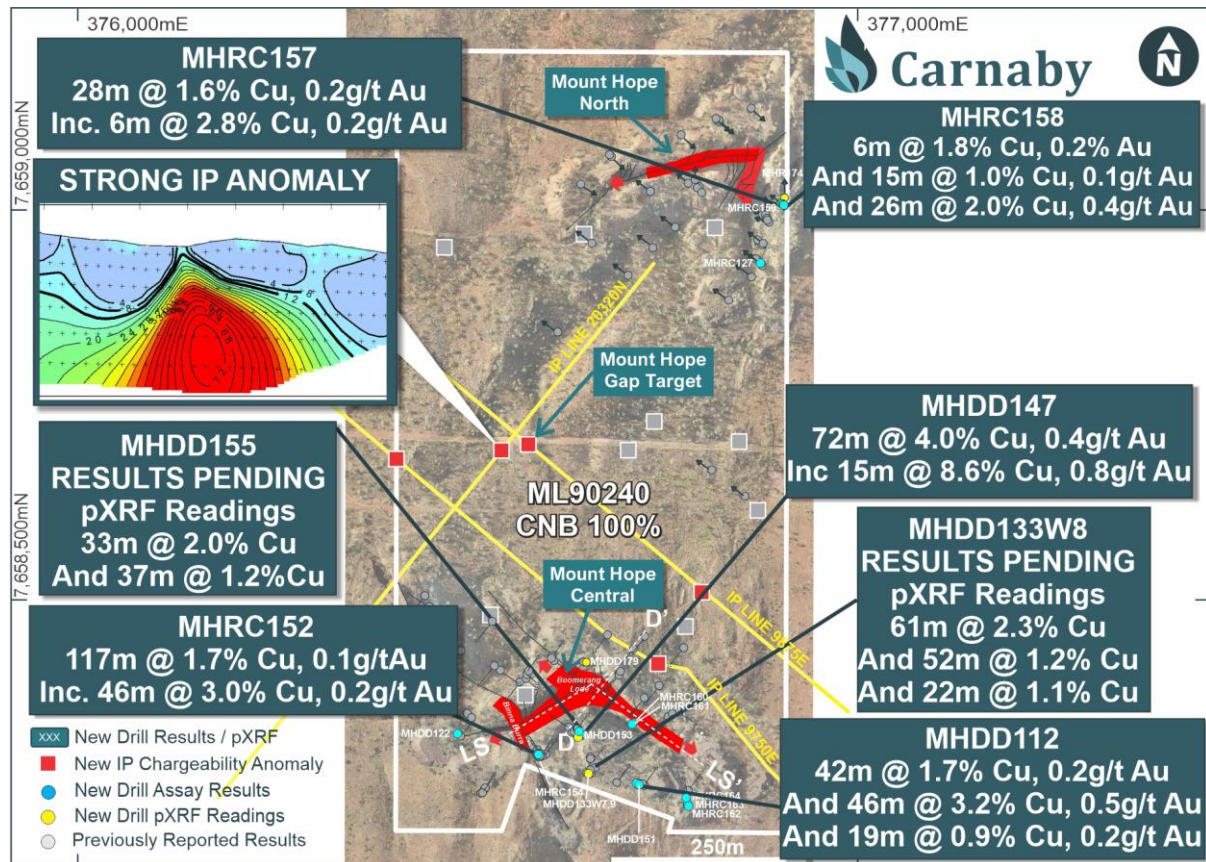
Figure 1. Mount Hope Plan Showing New IP anomaly and Drill Results.
