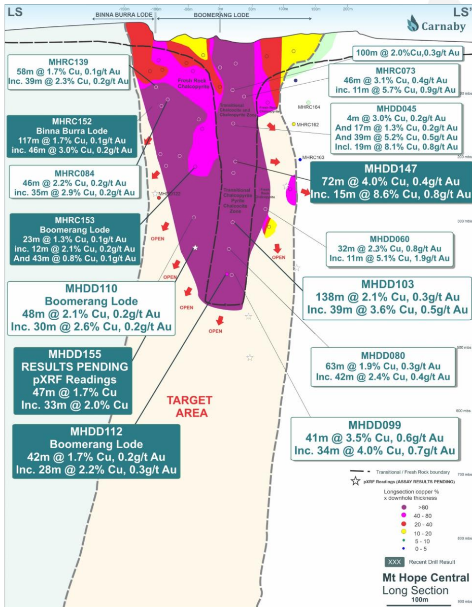
Figure 5. Mount Hope Central Boomerang Lode Long Section.
