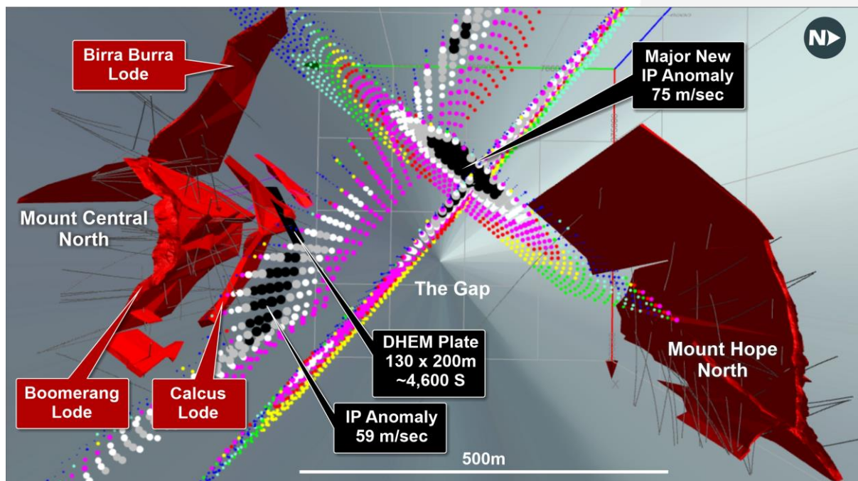
Figure 3. Mount Hope Plan Showing New IP anomaly and Drill Results.
