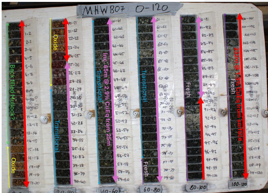
Figure 3. MHWB007 RC drill chip photos.
