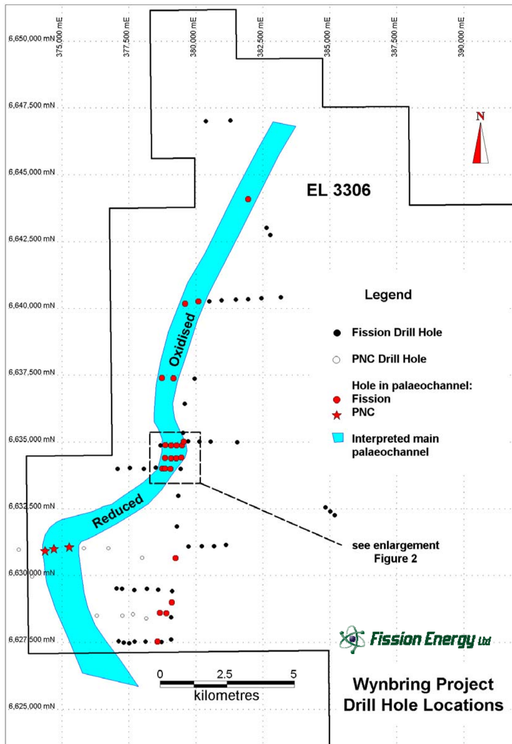
Figure 1: Drill Hole Locations and Interpreted Fluvial Channel Location
