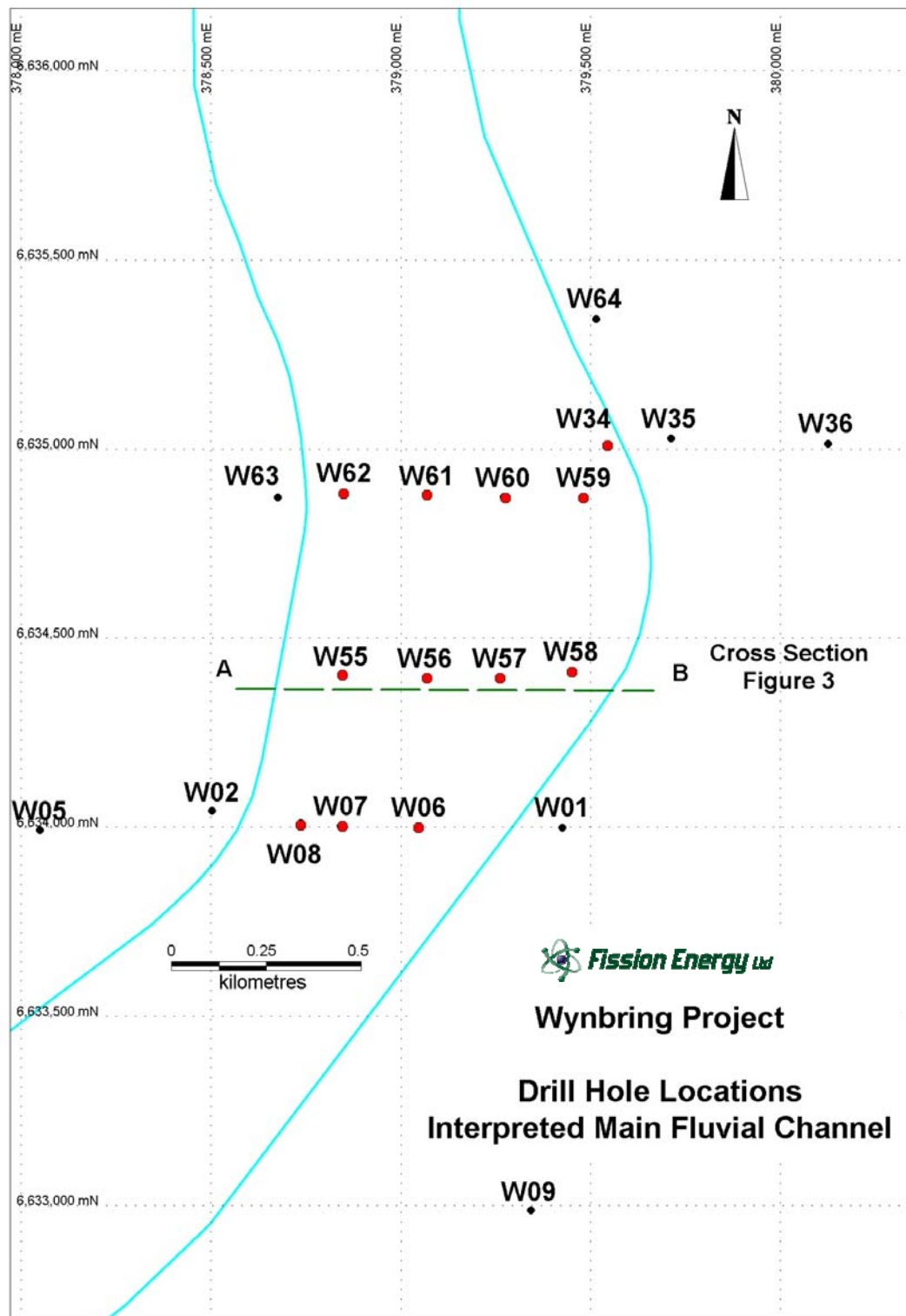
Figure 2: Drill Hole Locations Enlargement
