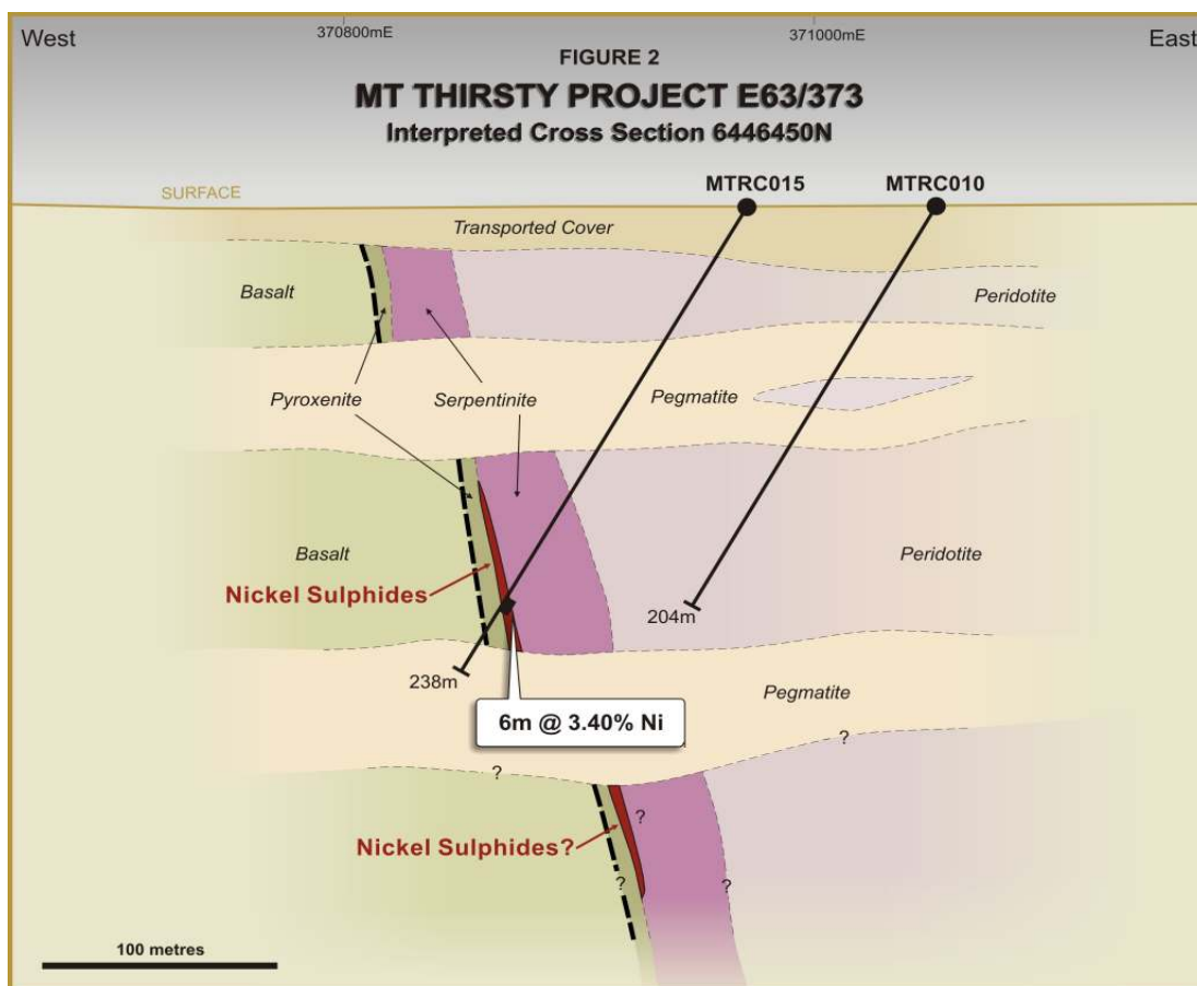
FIGURE 2: Mt Thirsty Project E63/373 Interpreted Cross Section.
