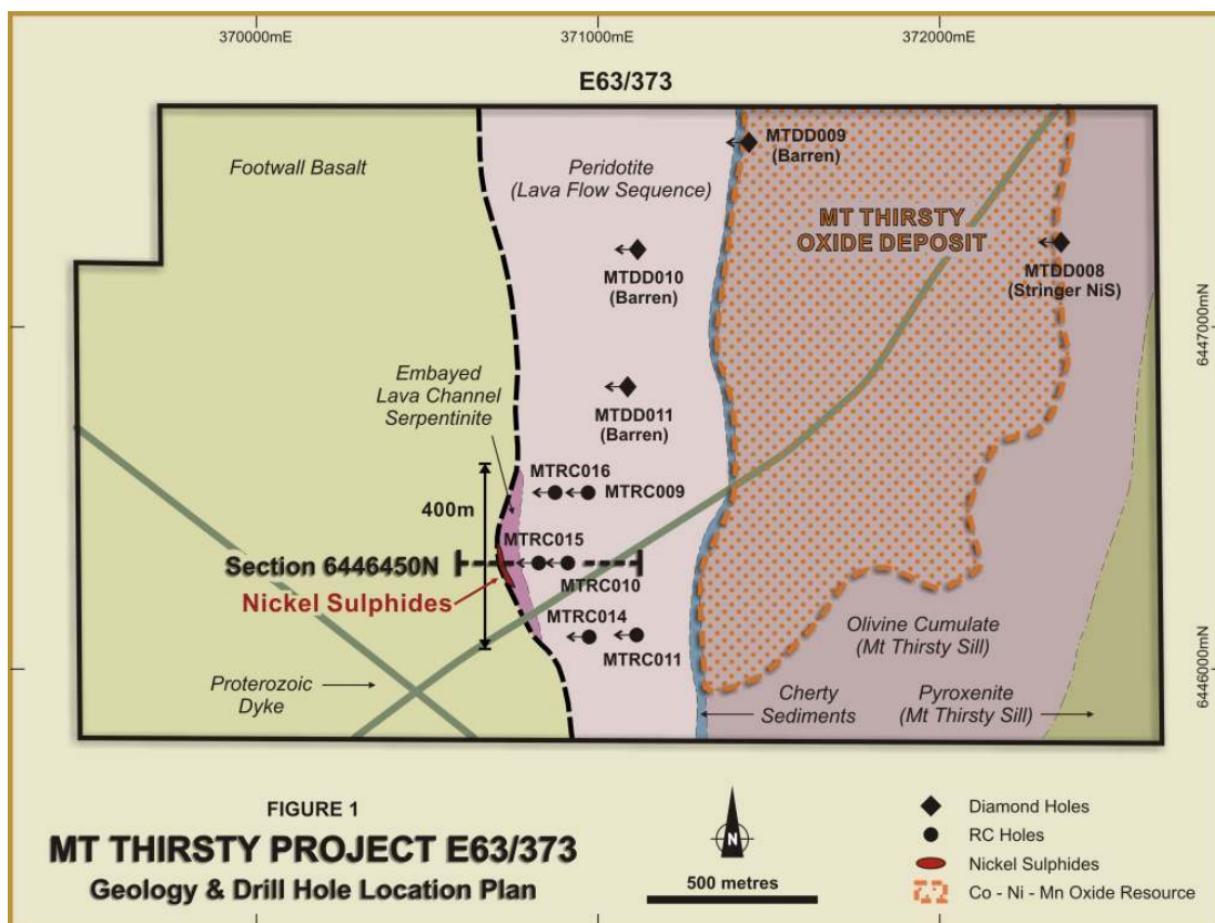
FIGURE 1: Geology and Drillhole Location Plan.
