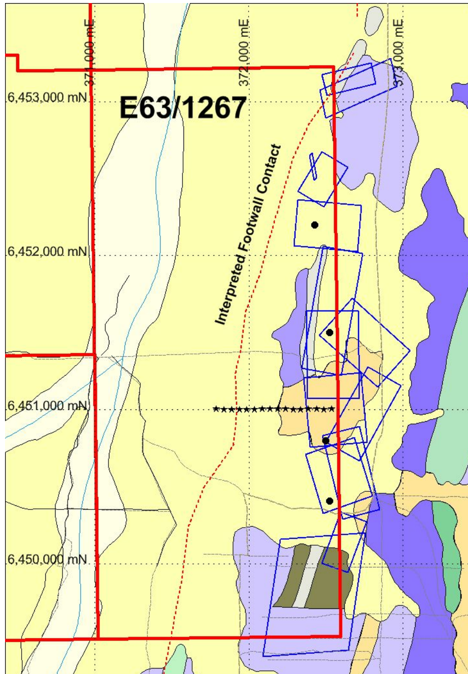
Figure 2: E63/1267, Planned air core drilling traverse (black stars), modelled EM conductors (blue rectangles) over GSWA mapping. The laterite target is coloured brown (GDA94, Zone 51).
