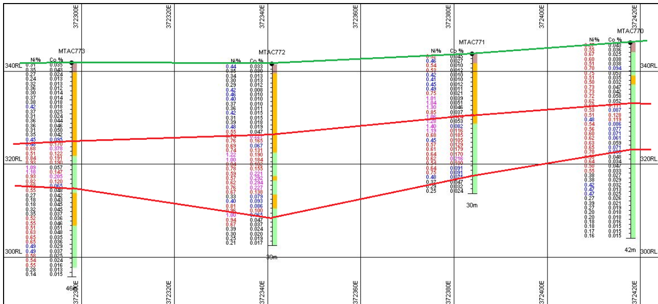
Figure 5: Cross Section A-B, 6451050N, looking north through holes MTAC770 to 773. Brown hatch is laterite, orange is goethitic saprolite and green is nontronitic saprolite. Ni% assays on the left and Co% assays on the right.
