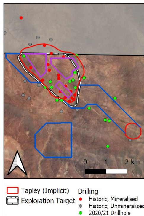
Figure 6: Map showing the current interpretation of known Tapley Hill Fm shale (red outline), the current Exploration Target outline (black and white outline) and drilling at the prospect (red, green and grey circles). Areas of proposed additional infill drilling are outlined in pink. Areas of possible extension/expansion are outlined in blue
