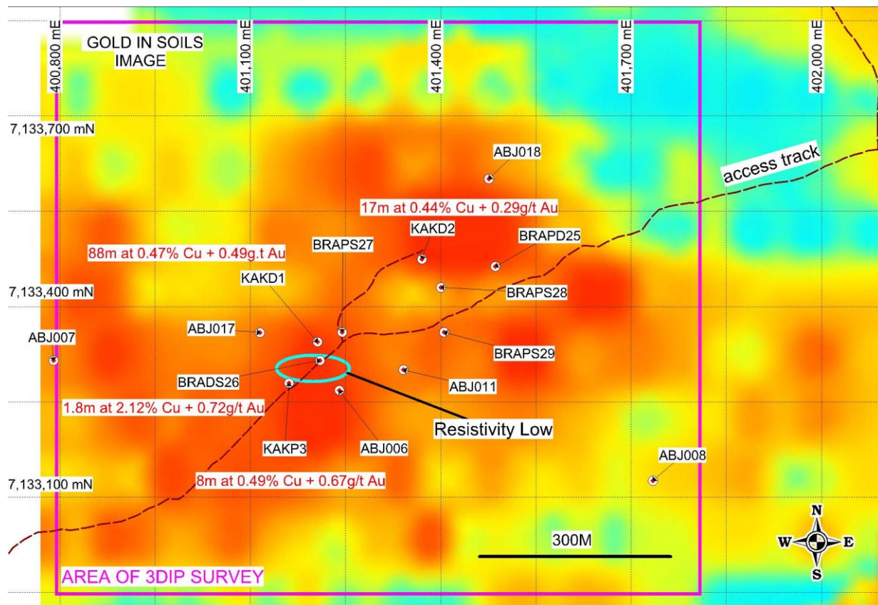
Figure 2: Kakapo drillholes, gold in soils grid and 3DIP survey area
