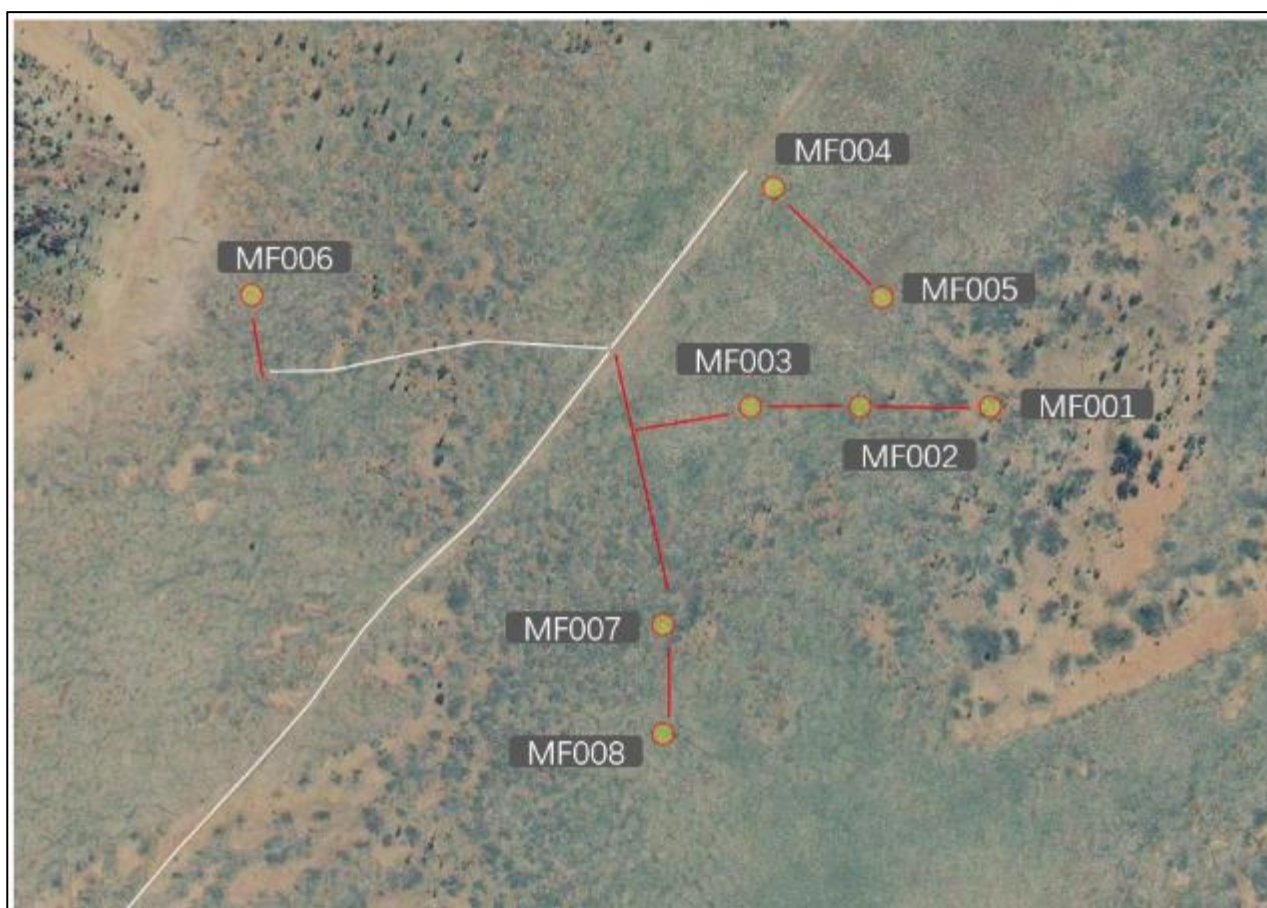
Figure 14: Location of diamond holes in Malakoff EPM 28853
