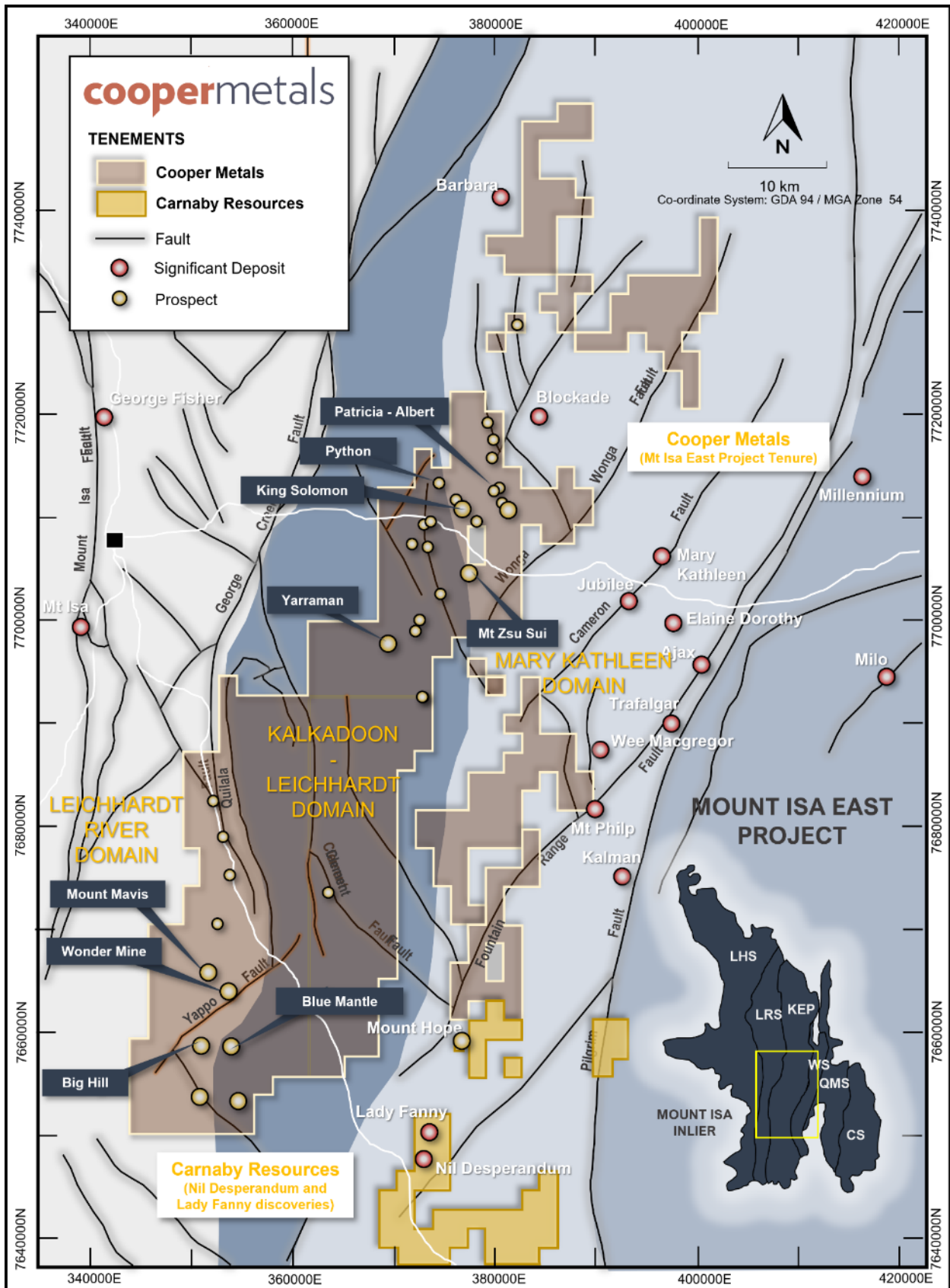
Figure 5: Mt Isa East Project Location Plan
