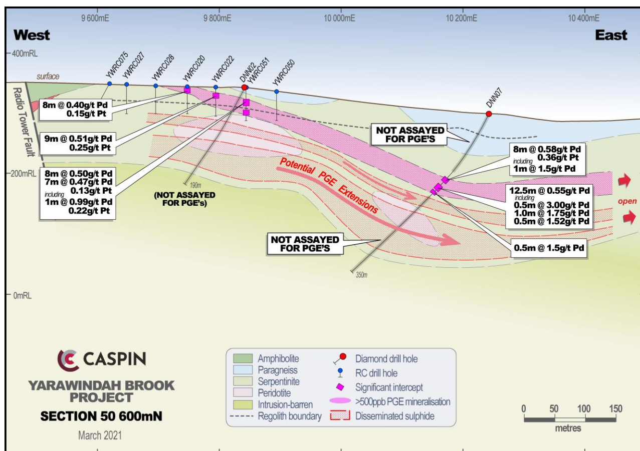
Figure 6. Section 50 600mN demonstrating PGE mineralisation extending into fresh rock but not effectively tested.
