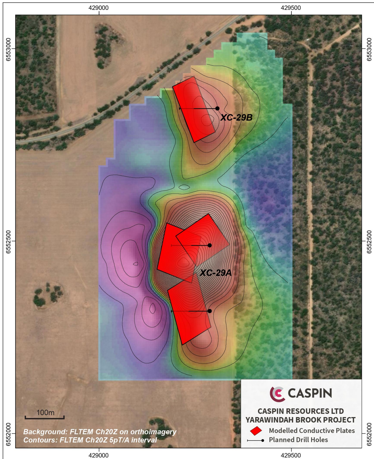
Figure 2. Modelled FLTEM conductors at XC-29a and XC-29b.
