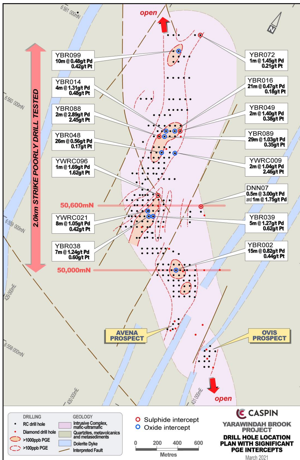
Figure 4. Collar plan and significant PGE assays.
