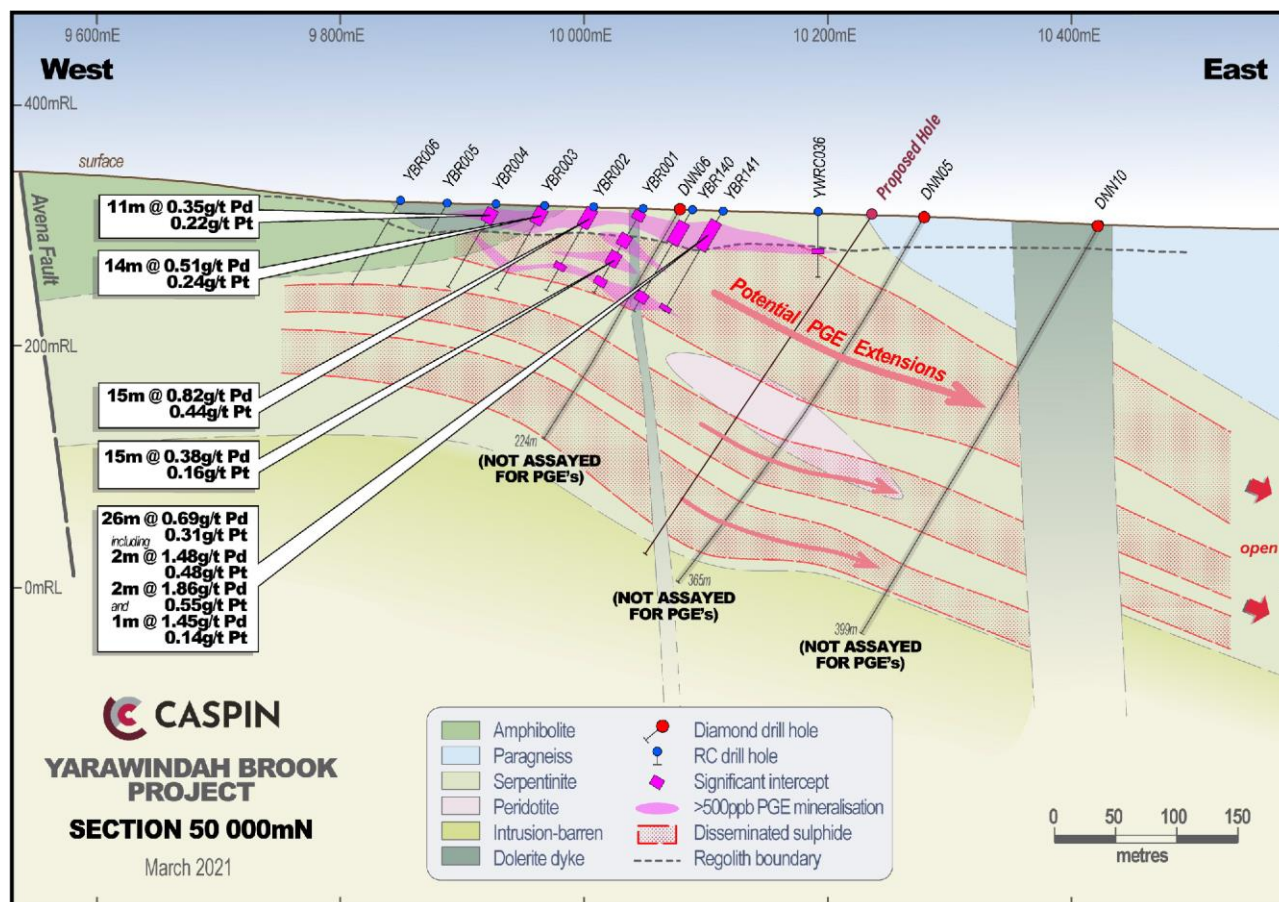
Figure 5. Section 50 000N demonstrating extensive surface mineralisation at surface and extending into fresh rock, but not assayed in deeper drill holes.
