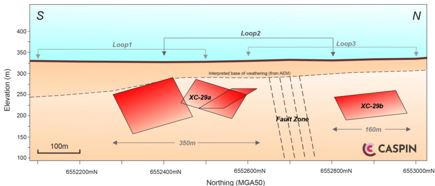
Figure 3. Long section through XC-29a & b showing geometry of FLTEM conductive plates.
