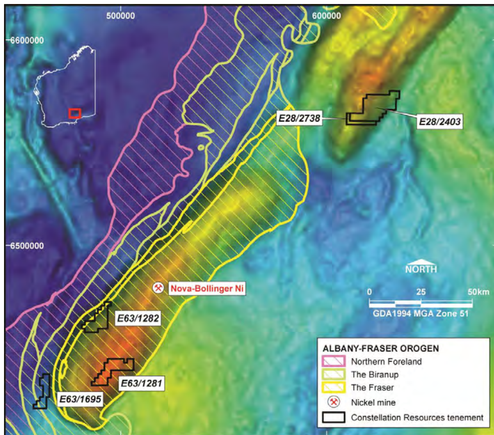
Figure 5: Location of the Nova-Bollinger deposit relative to the Project, highlighting the outcropping extent of rocks attributed to the Fraser Zone, largely interpreted from the regional gravity data
