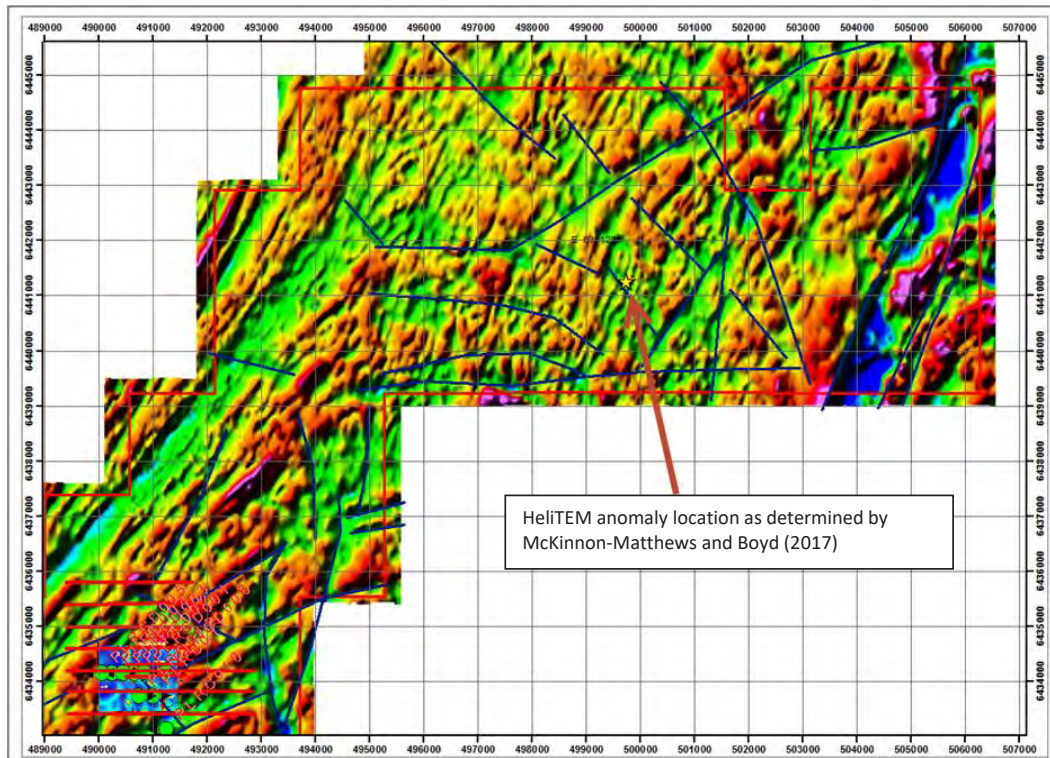
Figure 18: Location of HeliTEM anomaly on E63/1281 over airborne total field magnetic image and structural interpretation by McKinnon-Matthews and Boyd (2017)
