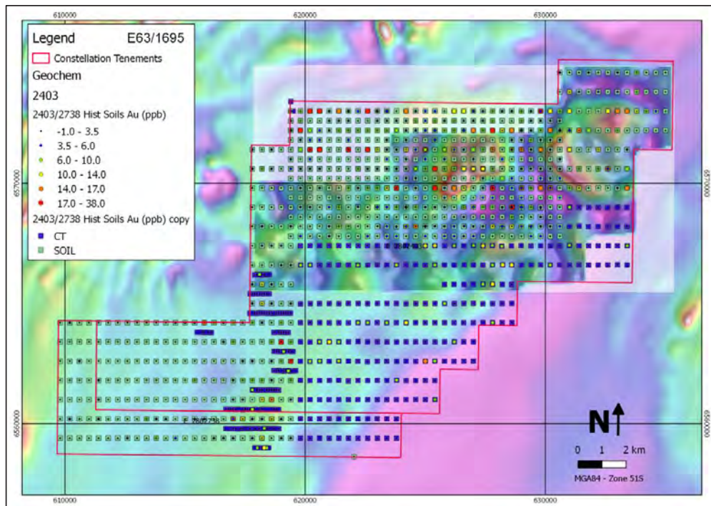
Figure 30: E28/2403 and E28/2738 showing surface sampling type (background points) and gold (ppb) (foreground points)
