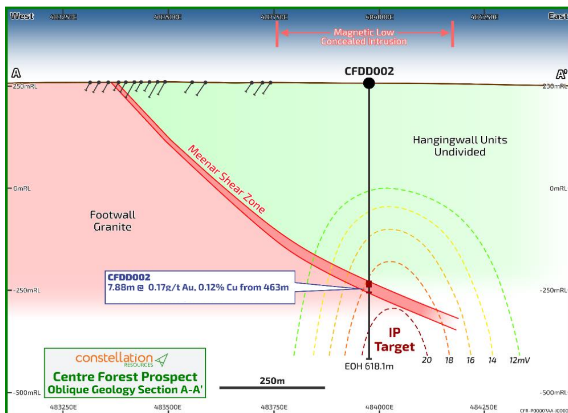
Figure 6: Simplified Centre Forest Cross Section A-A' showing CFDD002 drillhole intersection within the modelled chargeability anomaly
