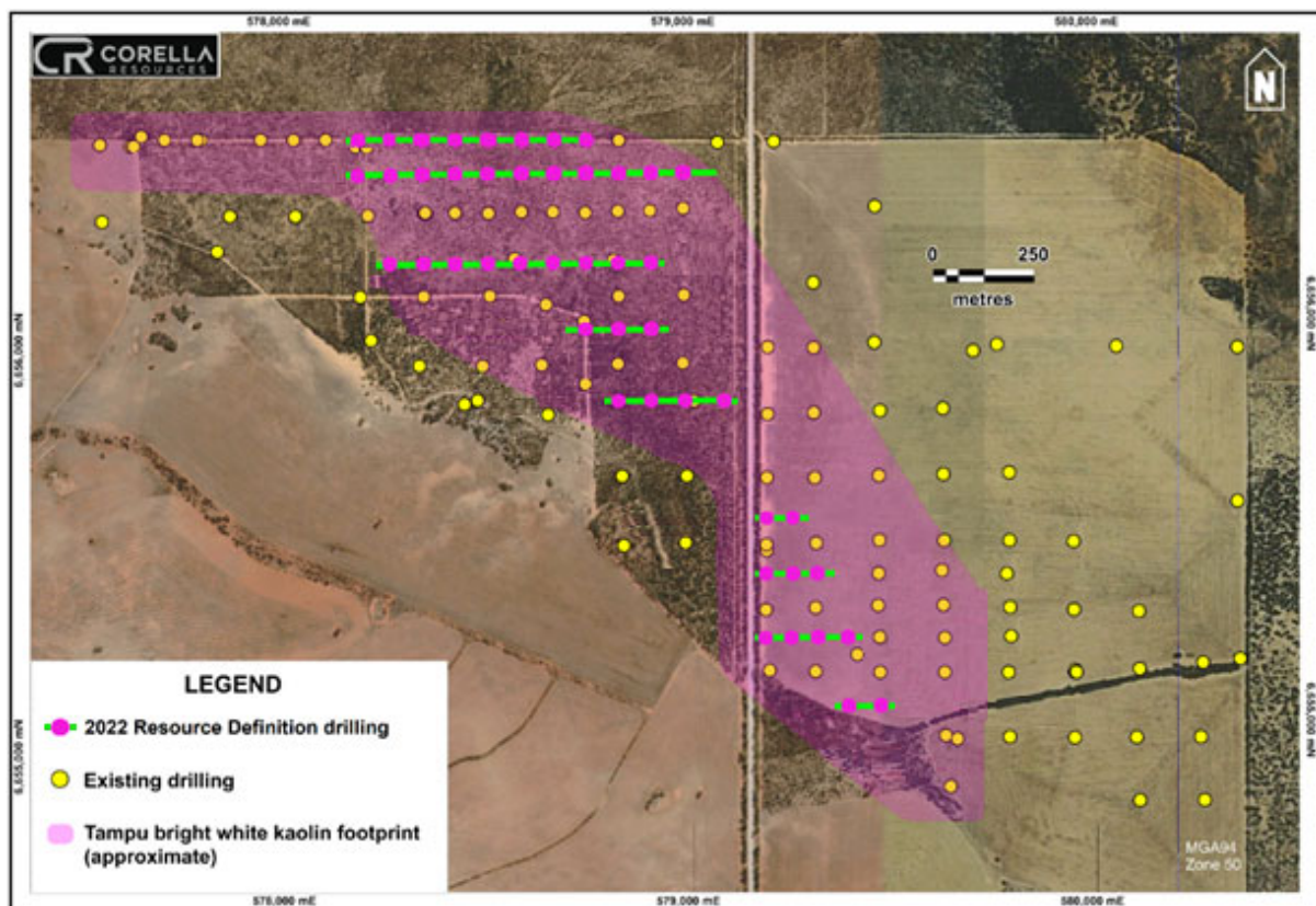
Figure 3: Recently completed Resource Definition drilling program at Tampu
