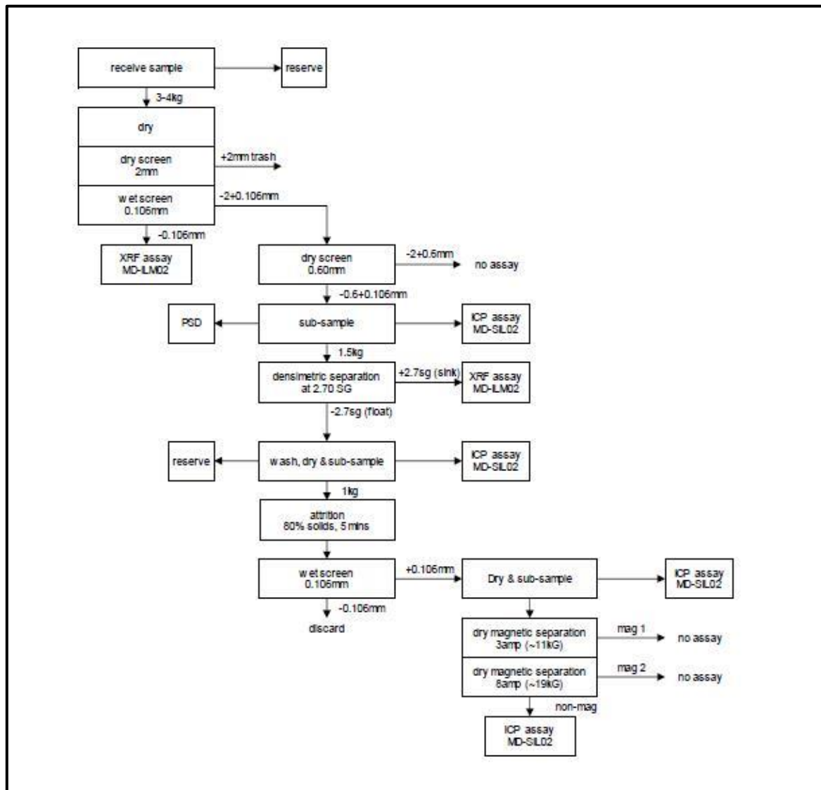
Figure 6: Processing Flowsheet
