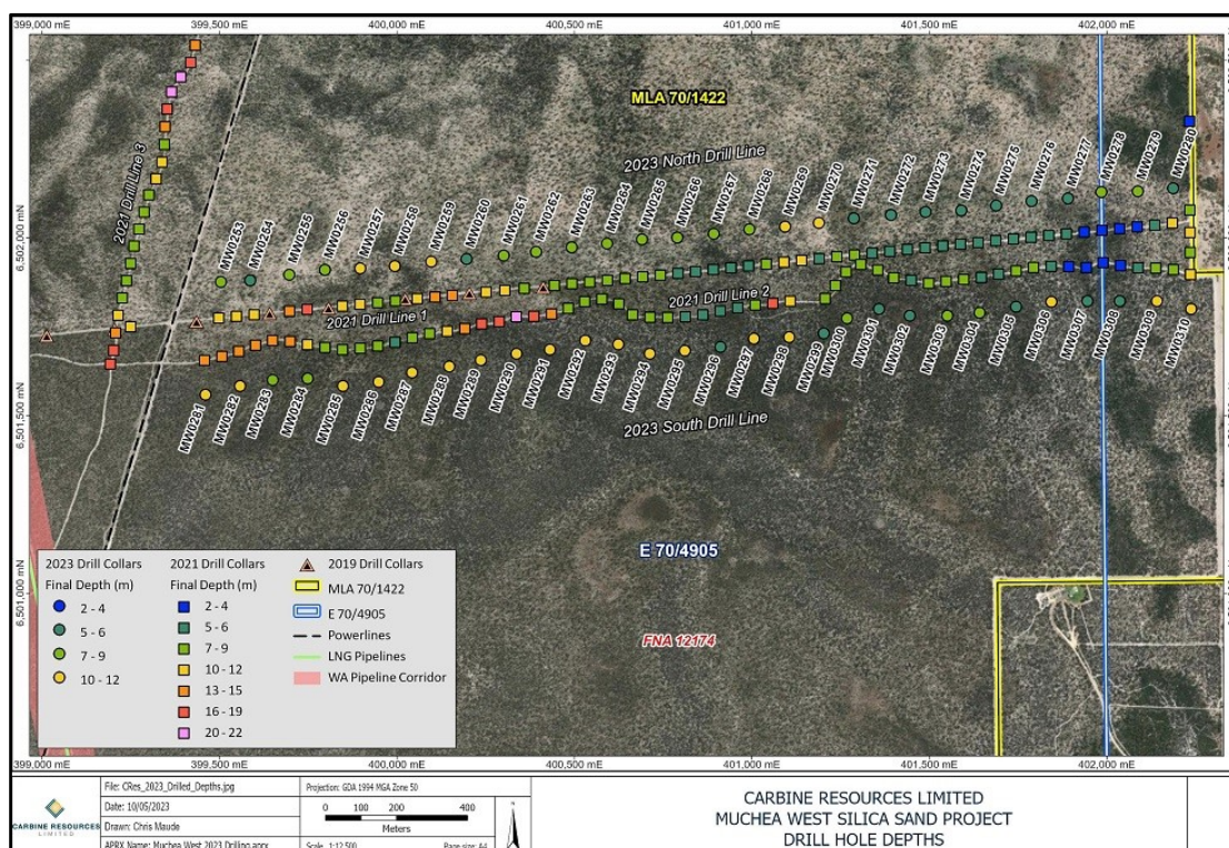
Figure 3: Drill spacings and depths
