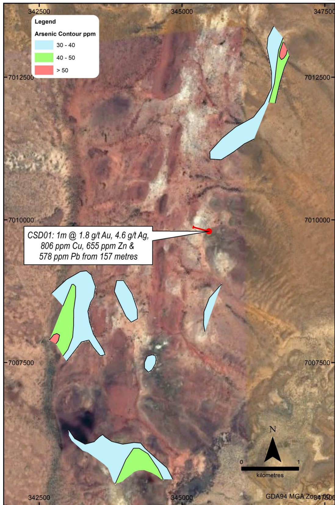
Figure Two | Caesar Project – Arsenic geochemical results
