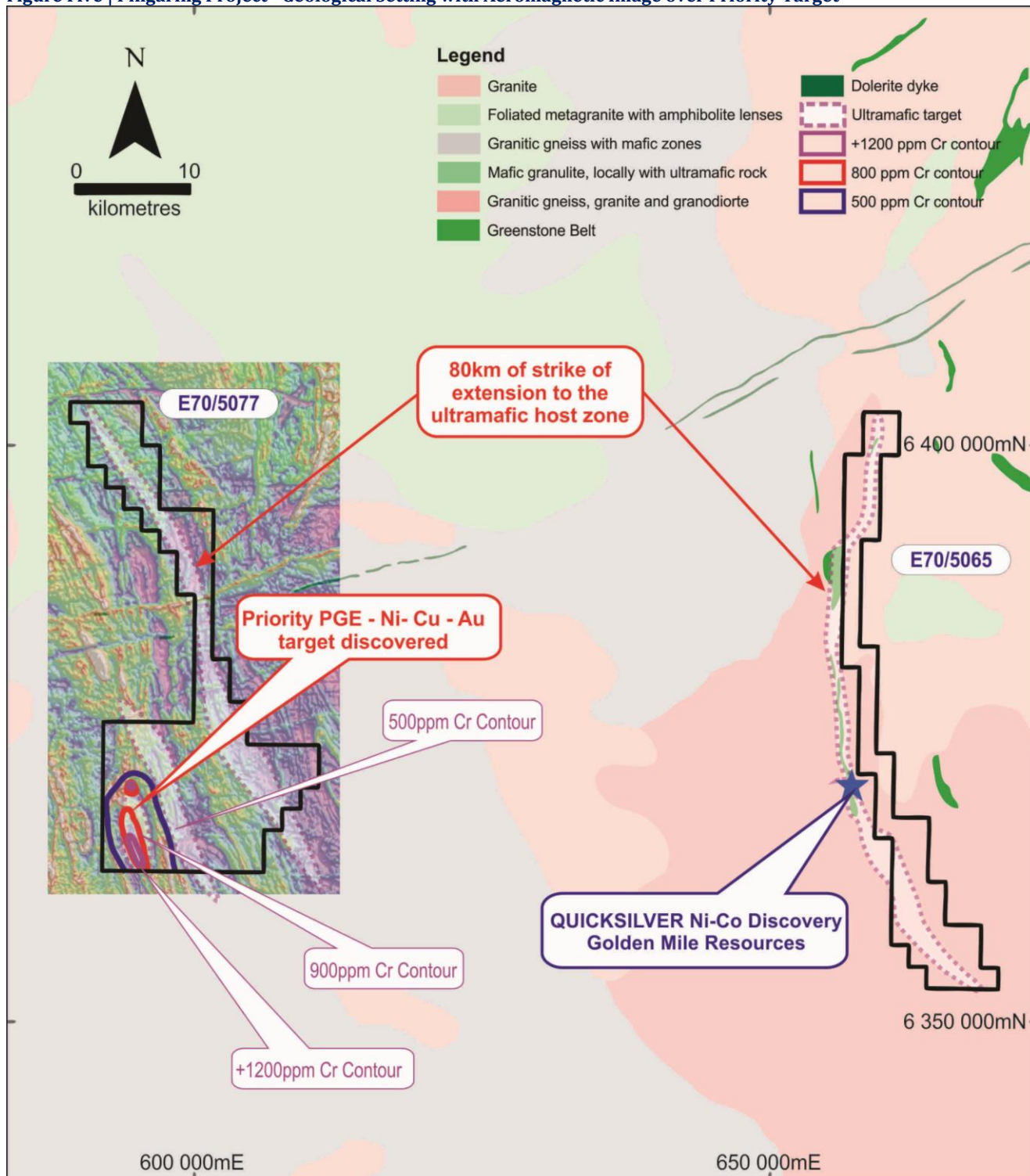
Figure Five | Pingaring Project - Geological Setting with Aeromagnetic Image over Priority Target
