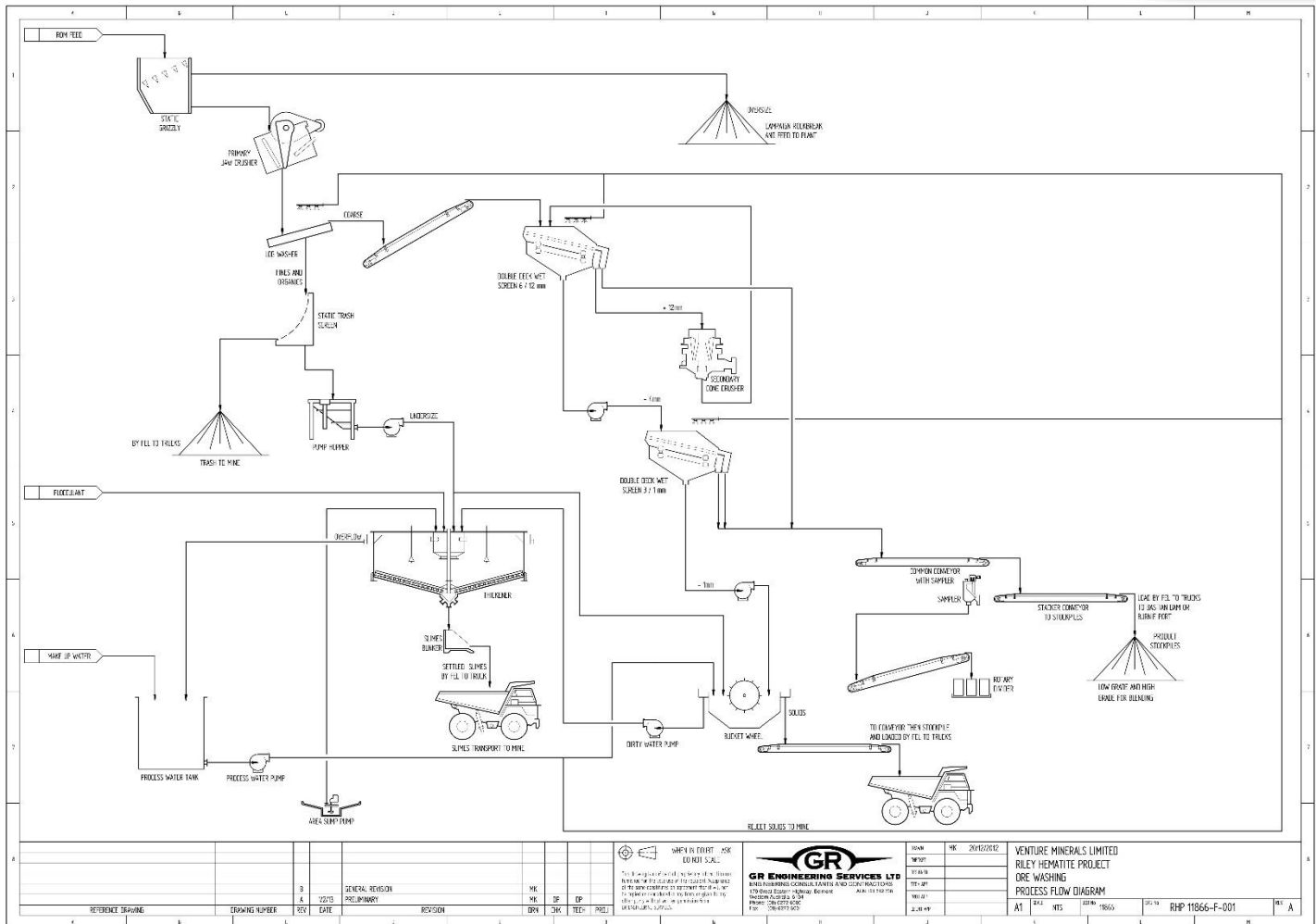
Figure 7: Ore Washing Process Flow Diagram
