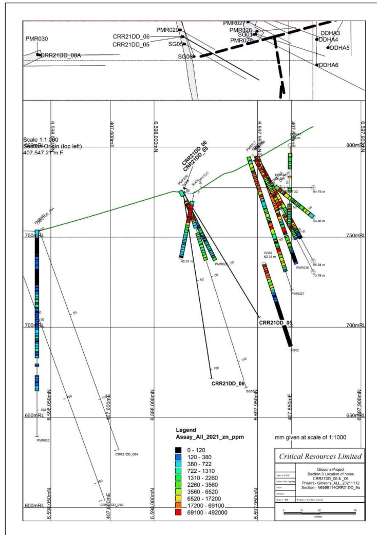
Figure 7- Drillhole CRR21DD_6 Cross Section
