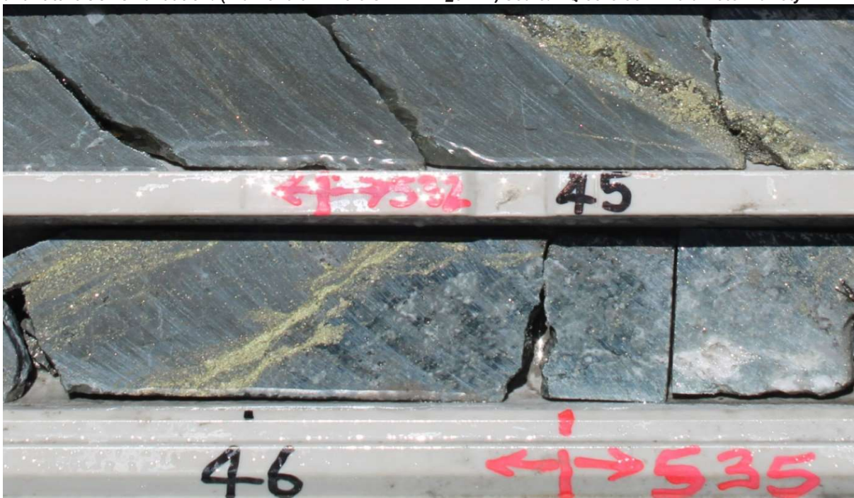
Figure 8: Half core from RHS of second and third row of Figure 7 above; note second row RHS sheeted, parallel vein (at the 45m downhole measurement) has chalcopyrite towards the central portion of the veins with more pyrite towards the margin; note third row RHS sheeted, parallel vein (at the 46m downhole measurement) is dominated by chalcopyrite. Note: Core is sawn in half:- half core sent for assay and half core retained for study and future JORC validation. (Diamond drill hole CRR21DD_011A, Scale: NQ core 50mm diameter variety)
