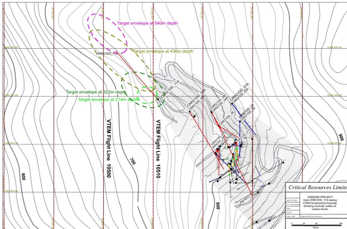
Figure 10: Gibsons project geophysical target outline at various levels (VTEM 2.5D processing)
