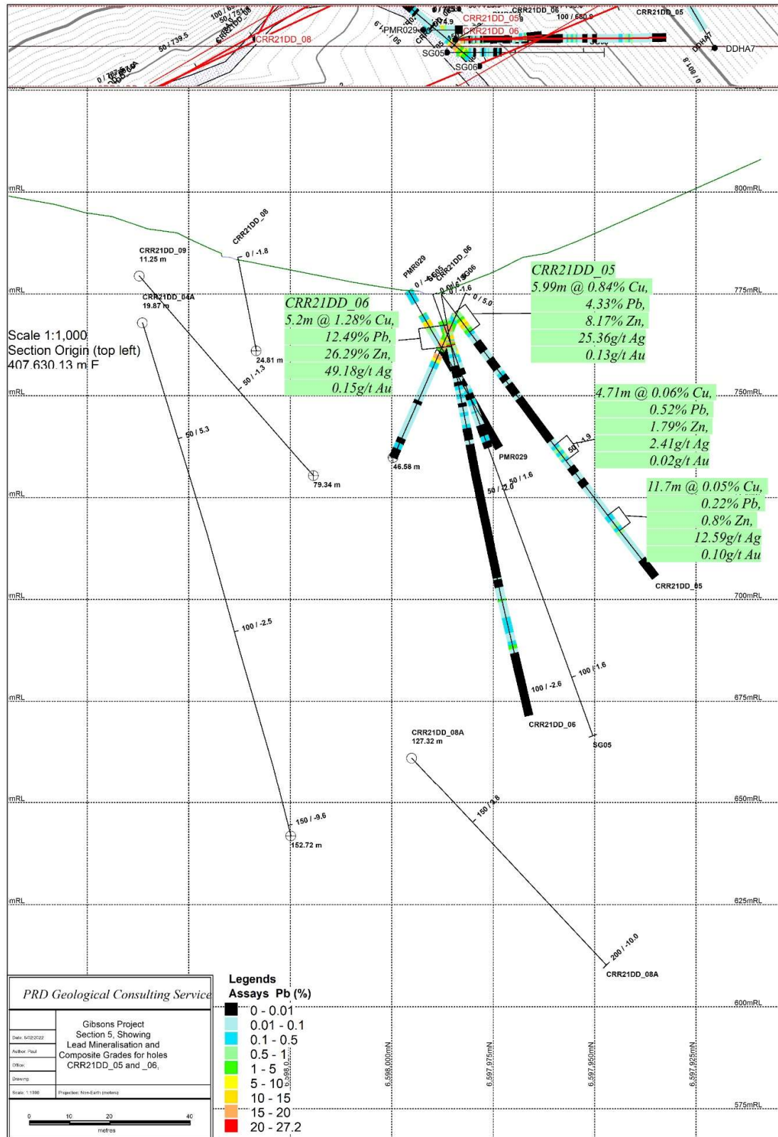
Figure 7: Cross-section and some downhole intersection, diamond drill hole CRR21DD21_05 and CRR21DD21_06
