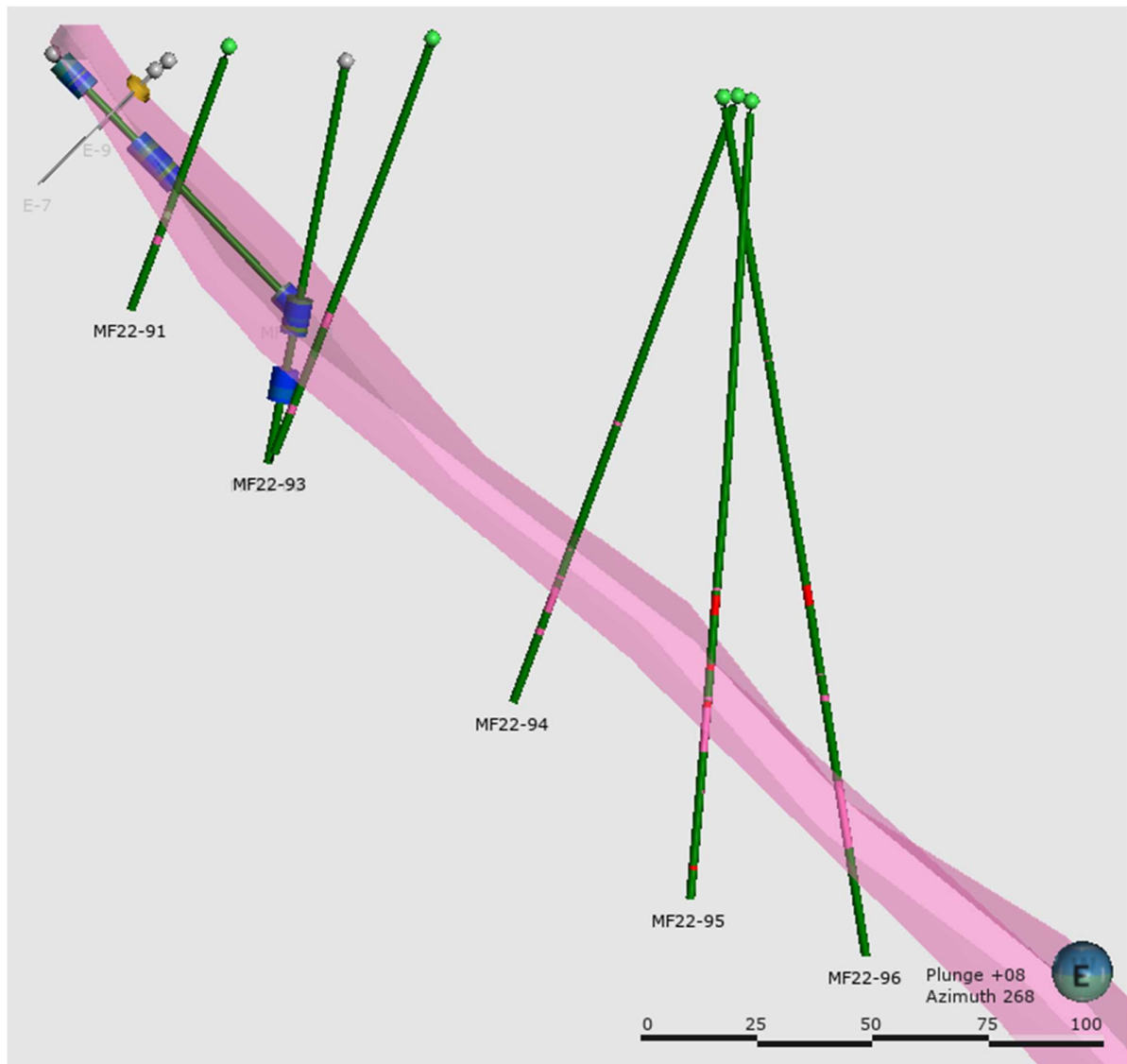
Figure 7: Cross-section, looking west, of Pegmatite 6 (pink shape) with previous drill hole traces (grey) and recently drilled holes of MF22-91, MF22-93, MF22-94, MF22-95, and MF22-96 (note: measurement in metres)
