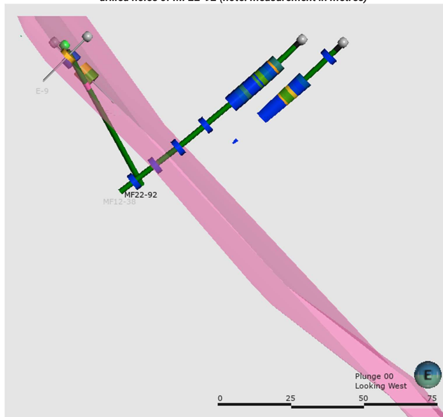
Figure 8: Cross-section, looking west, of Pegmatite 6 (pink shape) with previous drill hole traces (grey) and recently drilled holes of MF22-92 (note: measurement in metres)
