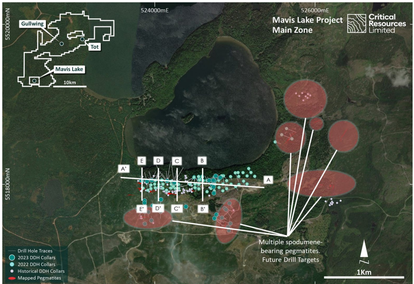
Figure 1: Plan Map of the Mavis Lake Main Zone and Cross Section references
