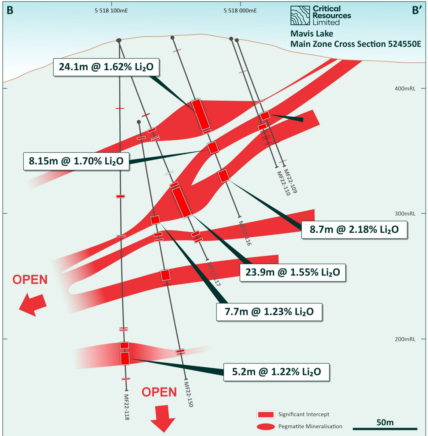
Figure 3: Section B-B' – Swell Zone near-surface
