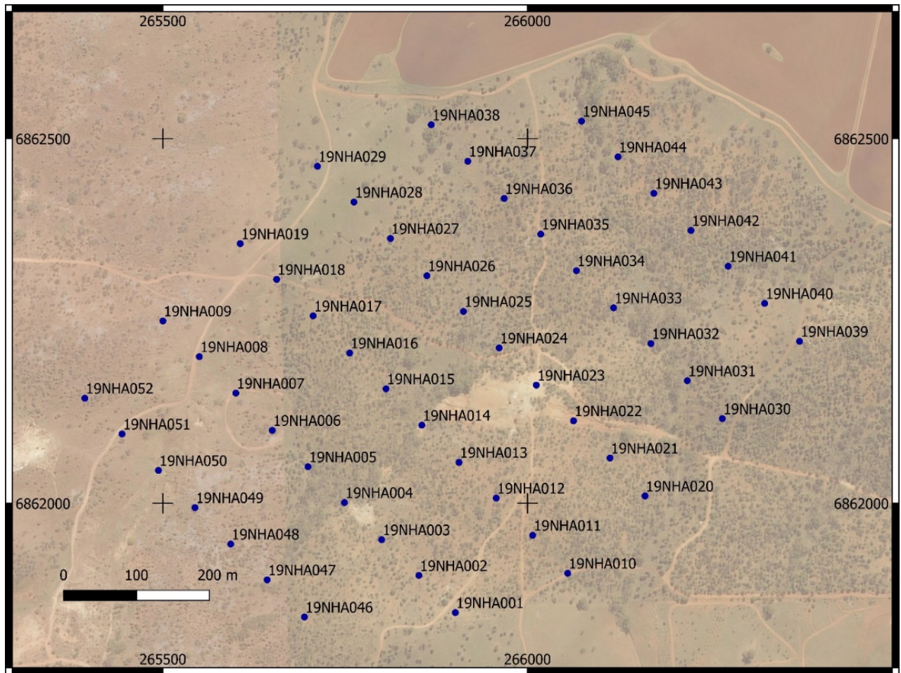
Figure 3: Detailed Auger Drill Collar Plan
