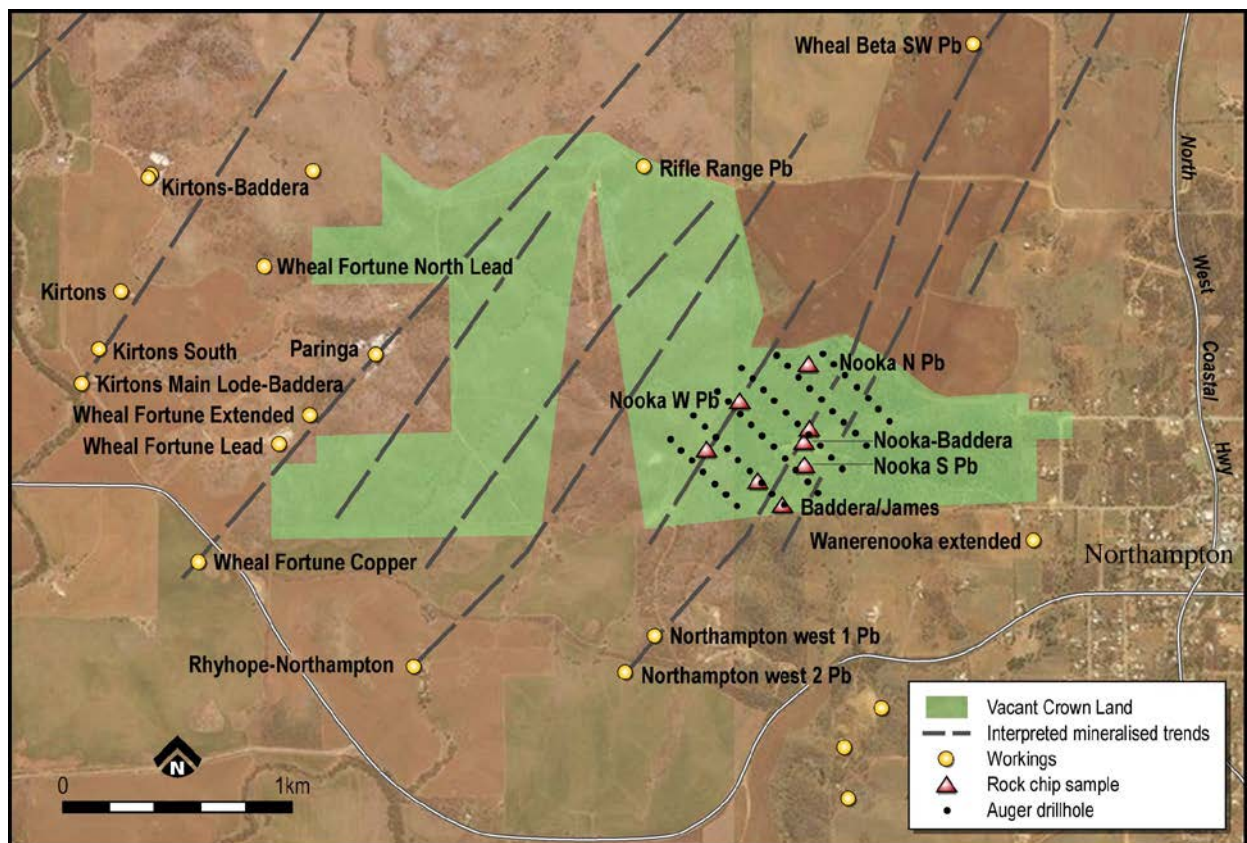
Figure 2: Location of Auger Drilling Holes
