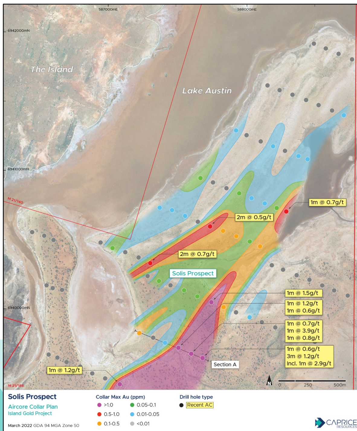
Figure 2: Solis aircore collar locations, coloured by Max Au in hole, with Max Au contours, updated to include the 1m resampling results.
