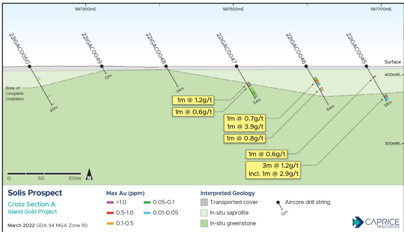
Figure 3: Solis aircore cross section A, see Figure 2 for section location, with all 1m sample intervals displayed
