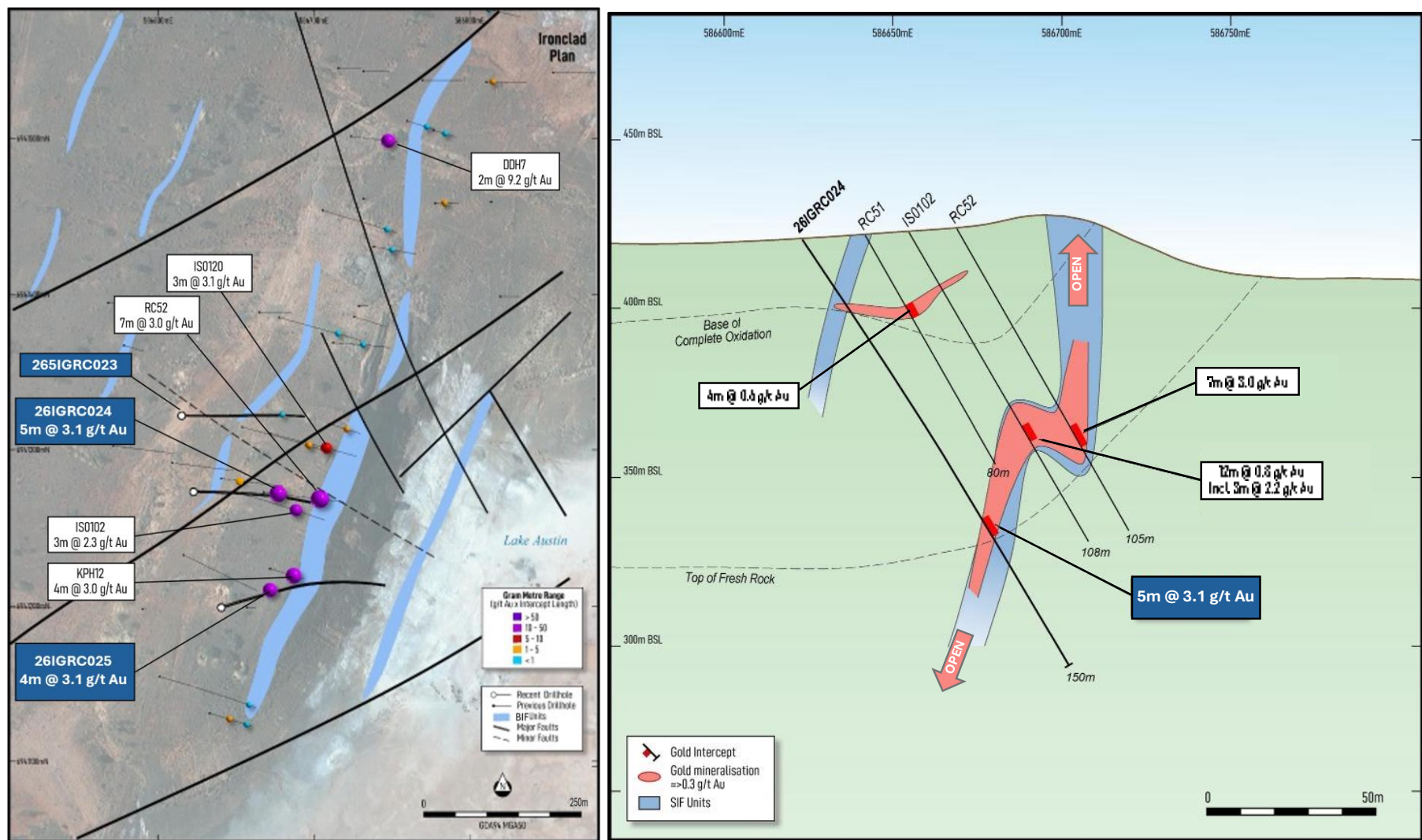
Figure 4: Schematic long section of Iron Clad gold deposit with geology exposed at surface (BIFs in blue) and highlighting recent significant drill results (blue boxes, white boxes indicate previously reported results).
