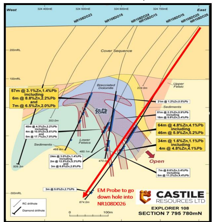
Figure 4: Explorer 108 DHEM Probe to survey for copper-rich anomalies beneath the lead/zinc deposit
