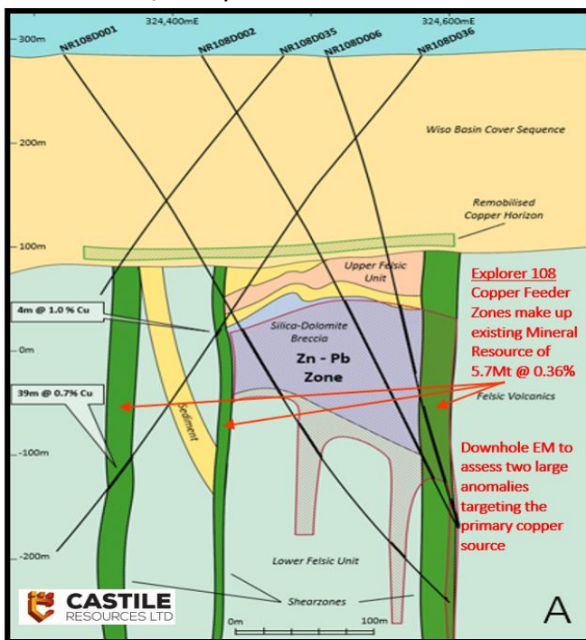
Figure 3: Explorer 108 Copper Feeder Zones surrounding the lead/zinc deposit
