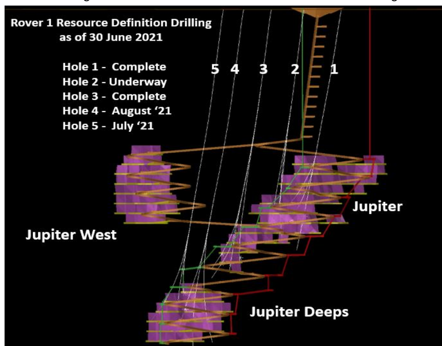
Figure 3: 2021 Rover 1 Resource Definition Drill Strings
