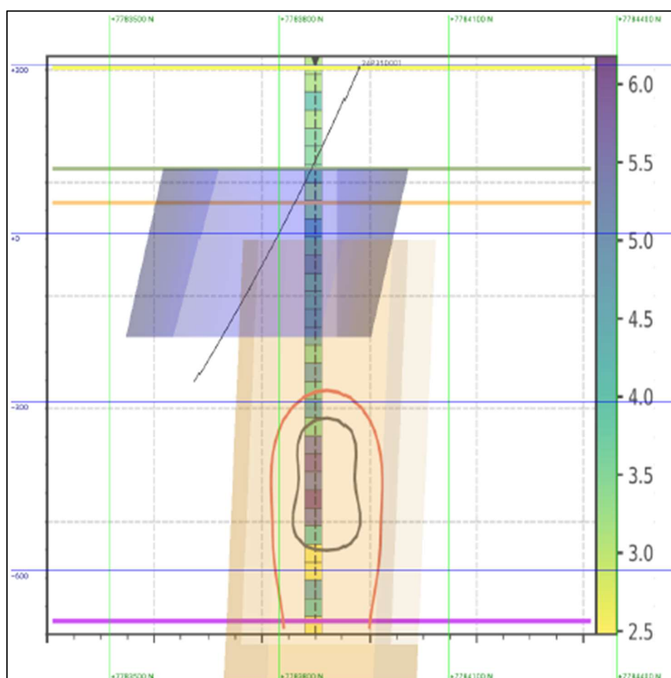
Figure 5: Pathfinder 35. Oblique section along ANT line showing station pair ANT inversions for P-wave velocity, remanent magnetic model (orange), non-remament original proposal magnetic model (blue) and original proposed diamond hole 24P35D001 from GDC1700004 in black.
