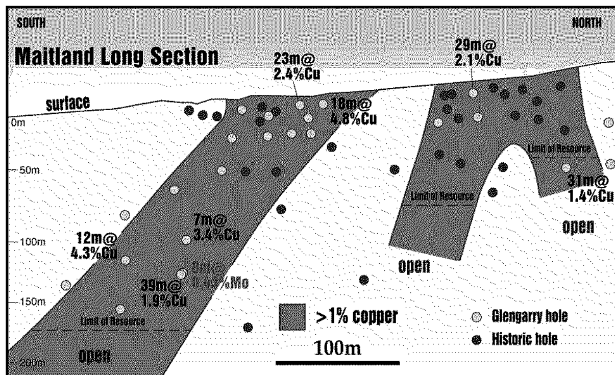
Figure 1: Maitland Long Section
