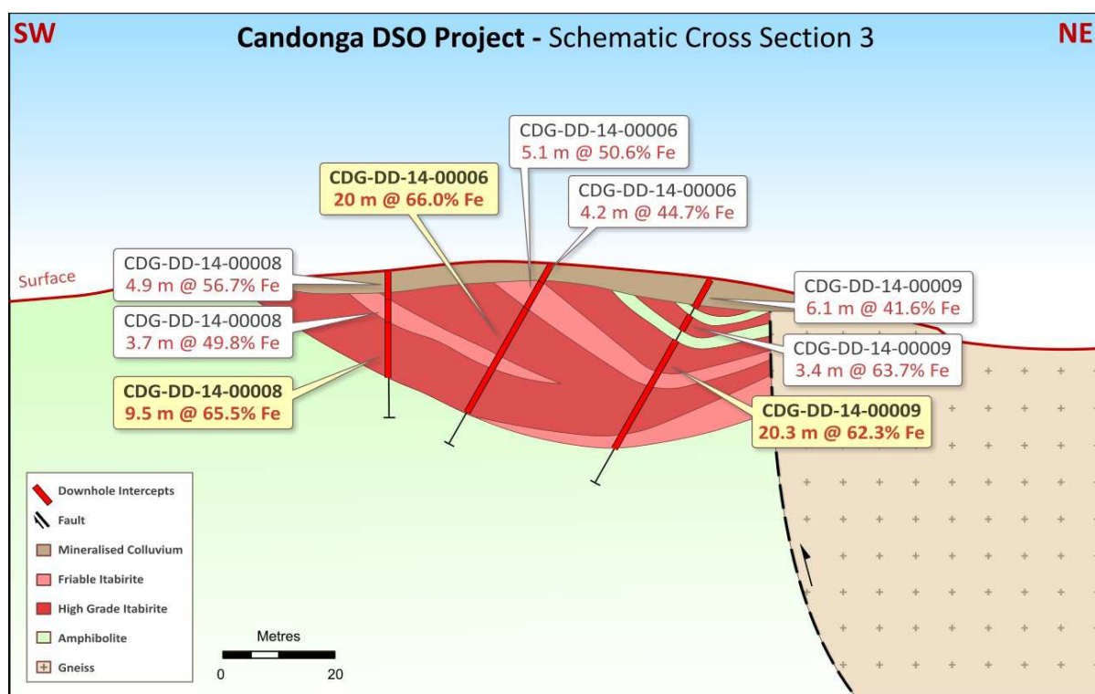
Figure 3 – Candonga Iron Ore Project – Schematic Cross Section 3
