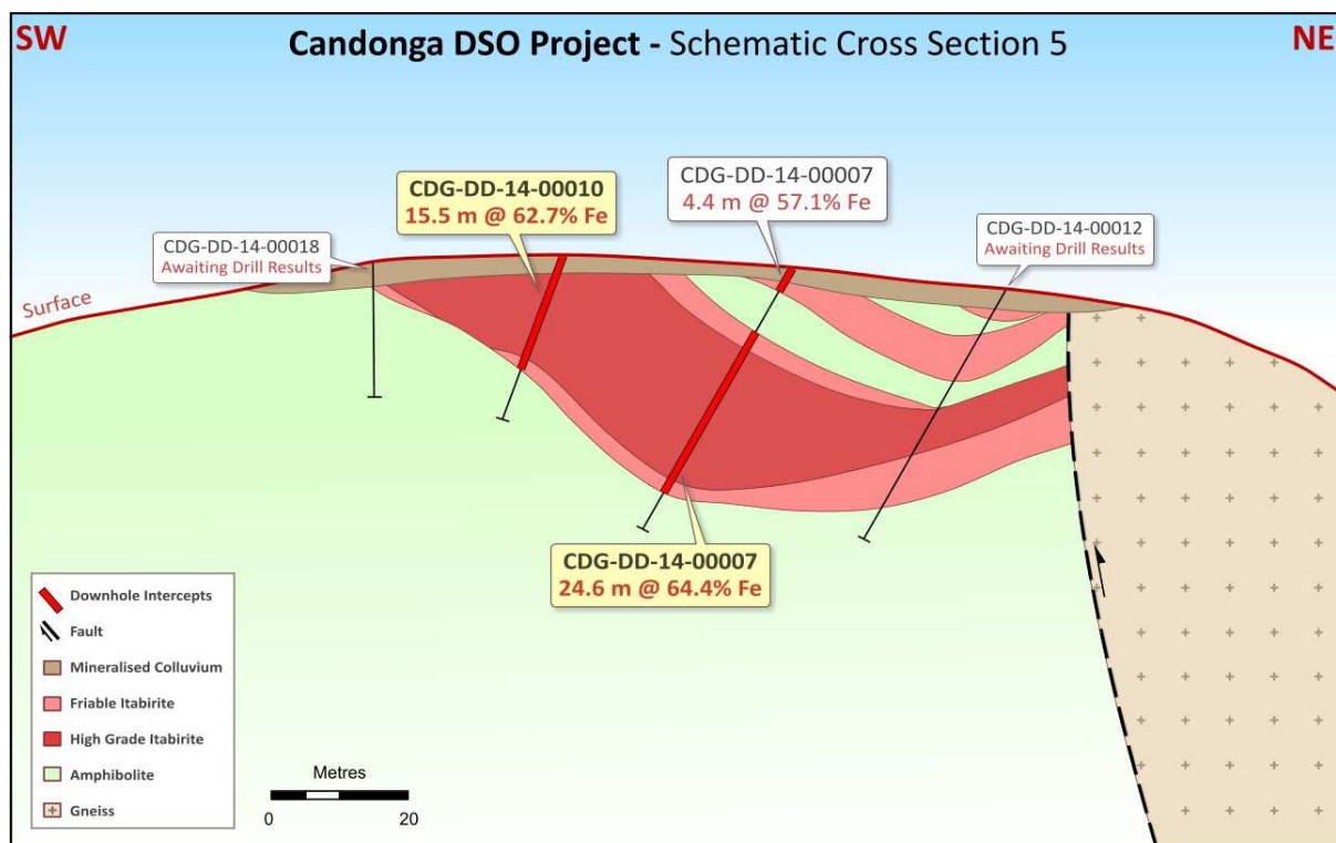
Figure 4 – Candonga Iron Ore Project – Schematic Cross Section 5
