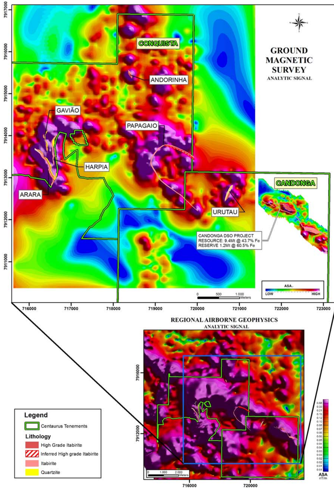
Figure 2: Conquista Project Ground Magnetic Survey, Analytic Signal 3
