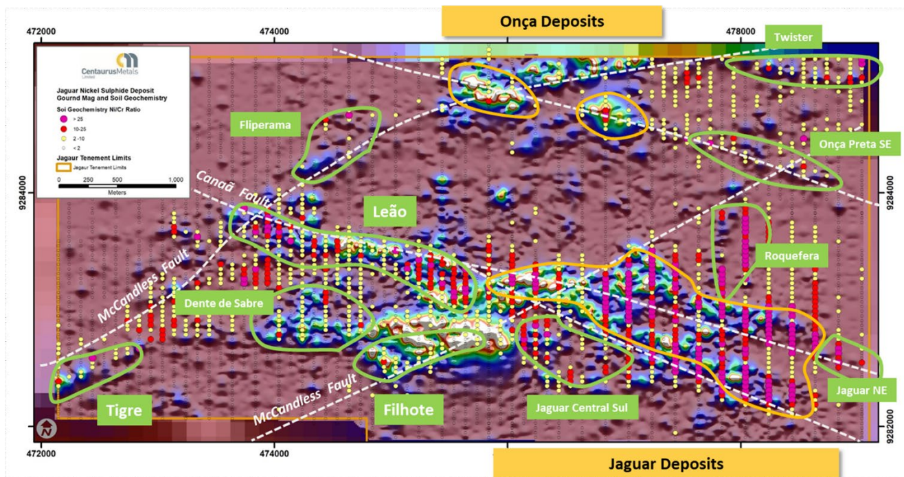
Figure 2 – The Jaguar Nickel Project – Soils Geochemistry (Ni/Cr) over Ground Magnetics (Analytic Signal)
