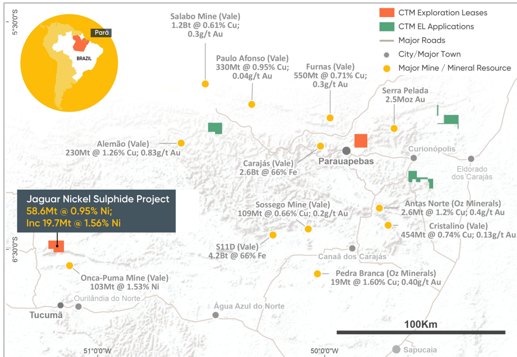
Figure 4 – The Jaguar Nickel Sulphide Project location.
