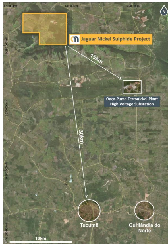
Figure 4 – The Jaguar Nickel Sulphide Project location.
