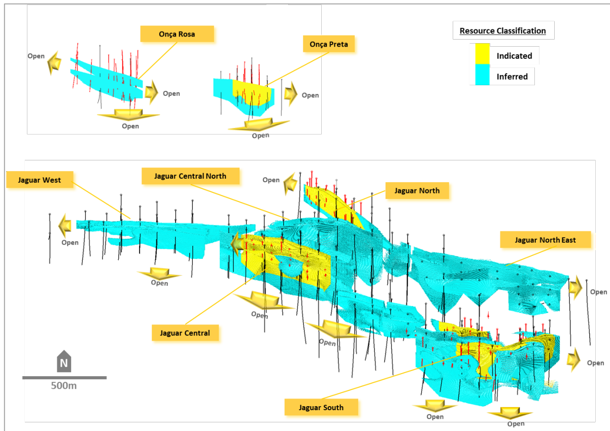
Figure 1 – The Jaguar MRE Block Model showing Resource Classification (Historical drilling shown in black; CTM drilling in red)
