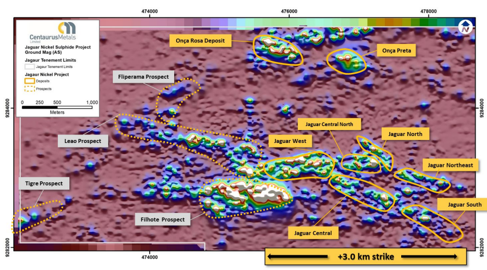
Figure 5 – Jaguar Nickel Project showing the various Deposits (yellow) and Prospects (grey) locations overlain on Ground Magnetics (Analytic Signal).
