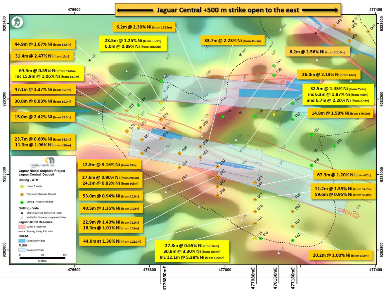
Figure 6 – The Jaguar Central Deposit with DHEM conductor plates (blue) overlaid on the Ground Magnetics Survey results (RTP) with location of the cross-sections shown.
