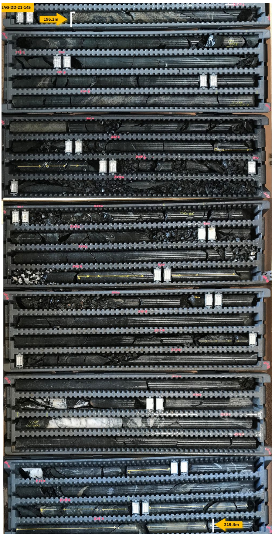
Figure 15 – Core photo from drill hole JAG-DD-21-145 (Jaguar Central); 196.2m to 219.4.9m down-hole: Disseminated, stringer to semi-massive sulphides (metallic bronze/yellow colour) with magnetite (black colour) mineralisation hosted in altered dacite. See Table 4 for sulphide content description.
