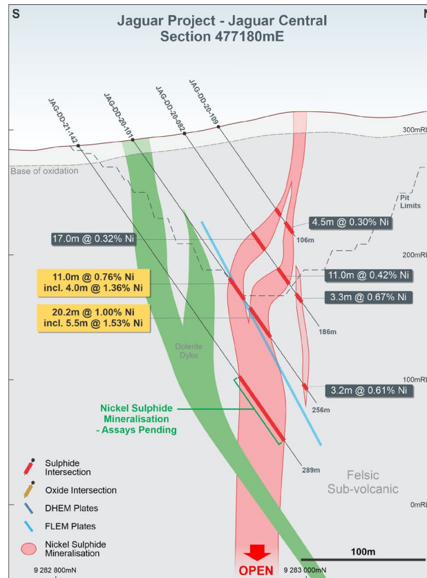
Figure 8 – The Jaguar Central Deposit: Cross-Section 477180mE showing the drill intersections with DHEM conductor plates in dark blue and FLEM plates in light blue.
