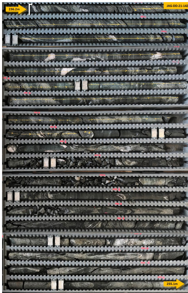
Figure 13 – Core photo from drill hole JAG-DD-21-142 (Jagaur Central); 236.2m to 255.1m down-hole: Disseminated, stringer to semi-massive sulphides (metallic bronze/yellow colour) with magnetite (black colour) mineralisation hosted in altered dacite. See Table 3 for sulphide content description.
