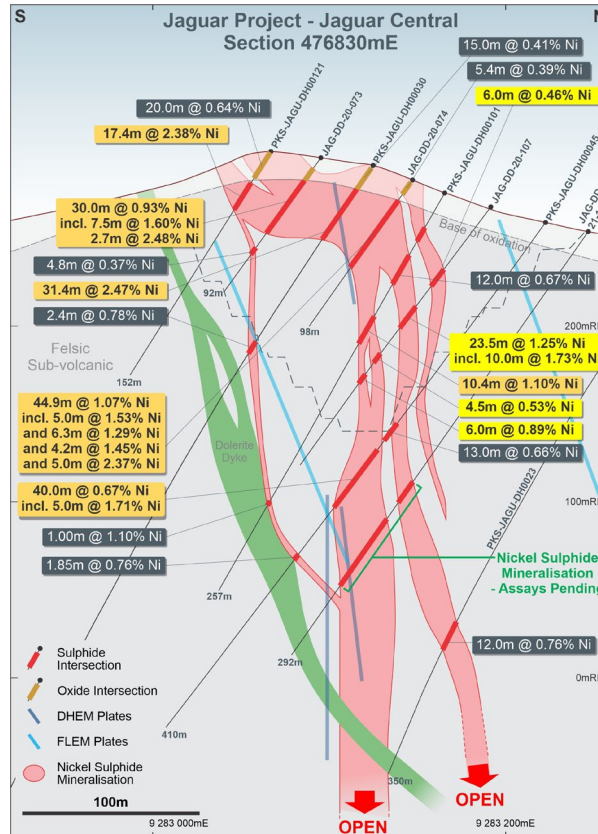
Figure 9 – The Jaguar Central Deposit: Cross-Section 476830mE showing the drill intersections with DHEM conductor plates in dark blue and FLEM plates in light blue.
