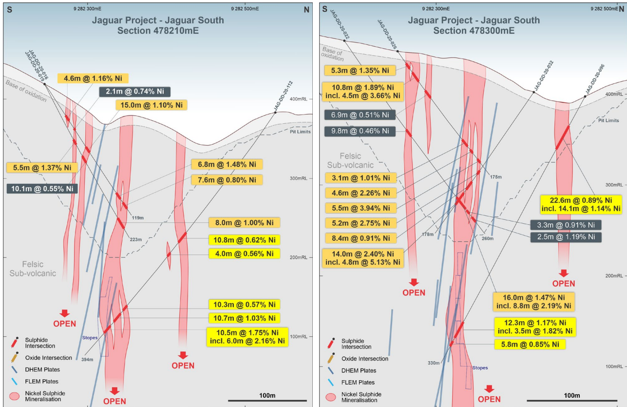
Figure 3 – The Jaguar South Deposit: Cross-Sections 478210mE (left) and 478300mE (right) showing significant drill intersections (in yellow) with DHEM conductor plates in blue.
