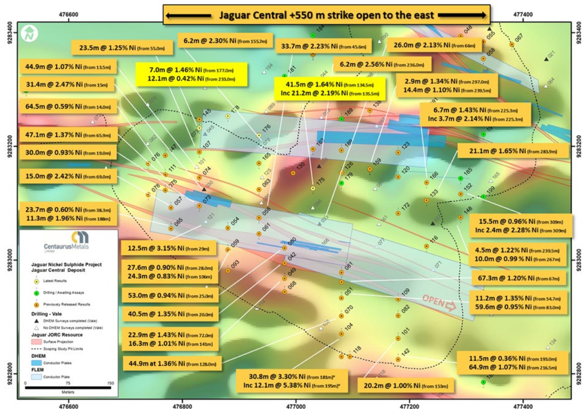
Figure 6 – The Jaguar Central Deposit with DHEM conductor plates (blue) overlaid on the Ground Magnetics Survey (RTP)
