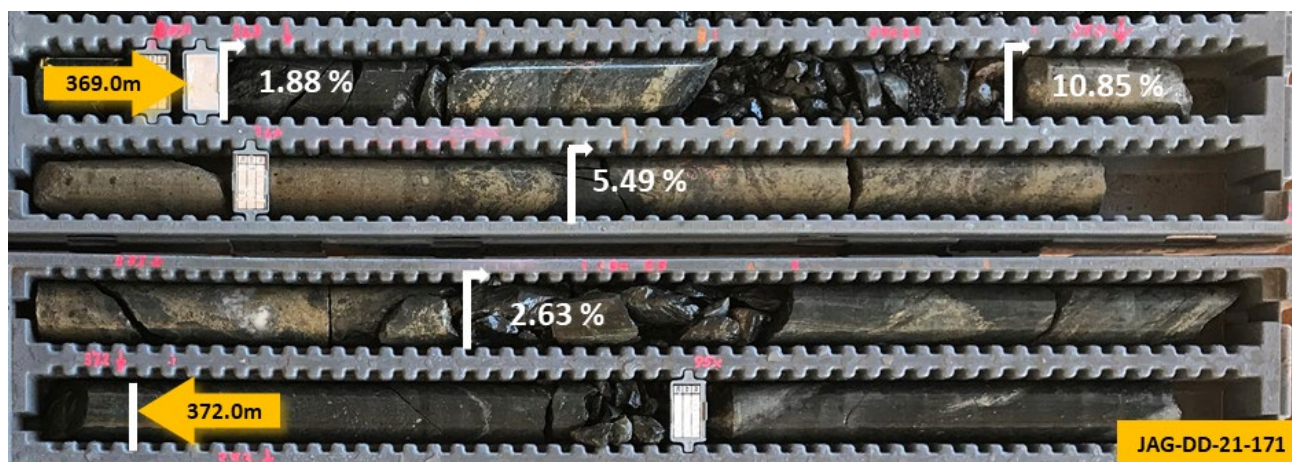
Figure 2 – Core photo from drill hole JAG-DD-21-171 (Jaguar South), 369.0m to 372.0m down-hole: Stringer to semi-massive and massive sulphides (metallic bronze/yellow colour) with magnetite (black colour) mineralisation hosted in altered dacite. This interval returned: 3.0m at 5.56% Ni from 369.0m and is part of a broader intersection of 21.0 at 1.25% Ni from 367.0m .
