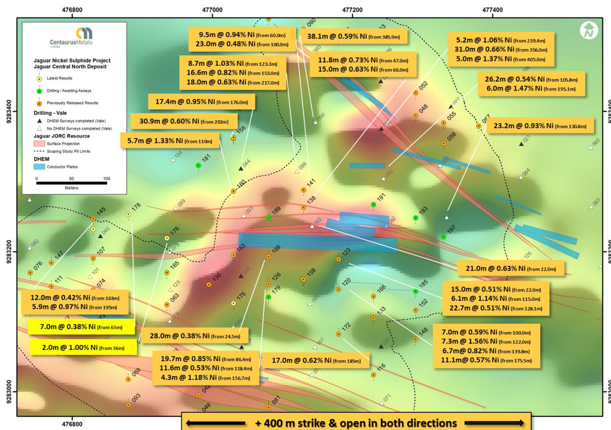
Figure 8 – The Jaguar Central North Deposit with DHEM conductor plates (blue) overlaid on the Ground Magnetics Survey (RTP)
