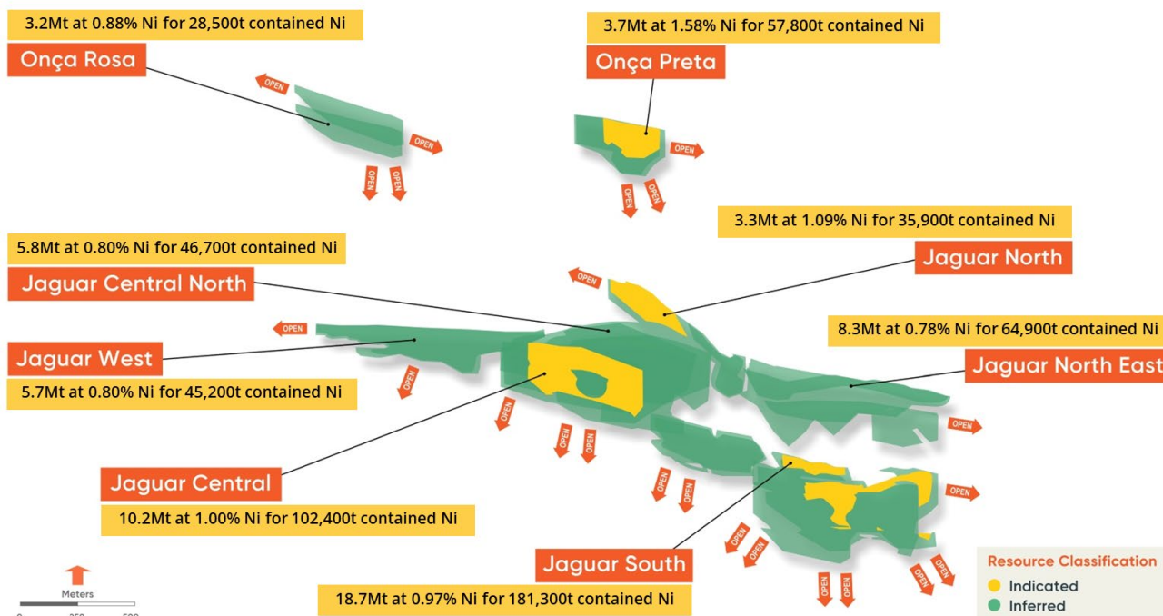
Figure 4 – The Jaguar March 2021 MRE Resource
