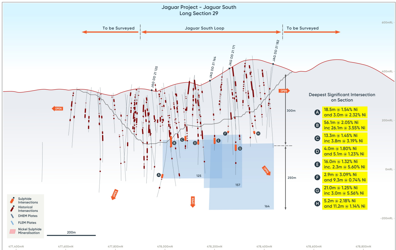
Figure 1 – The Jaguar South Deposit: Long-Section (looking north) showing the location of the new late-time (Ch20+) DHEM conductor plates below the current limit of drilling.
