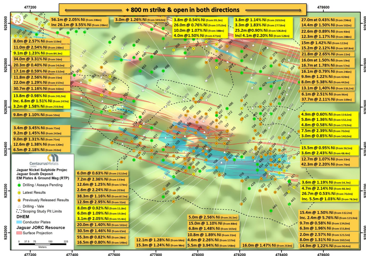
Figure 5 – The Jaguar South Deposit with DHEM (darker blue) and FLEM (lighter blue) conductor plates overlaid on the Ground Magnetism Survey results (Analytic Signal).
