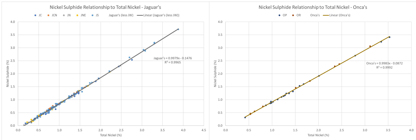
Figure 2: Total Nickel to Sulphide Nickel Relationship
