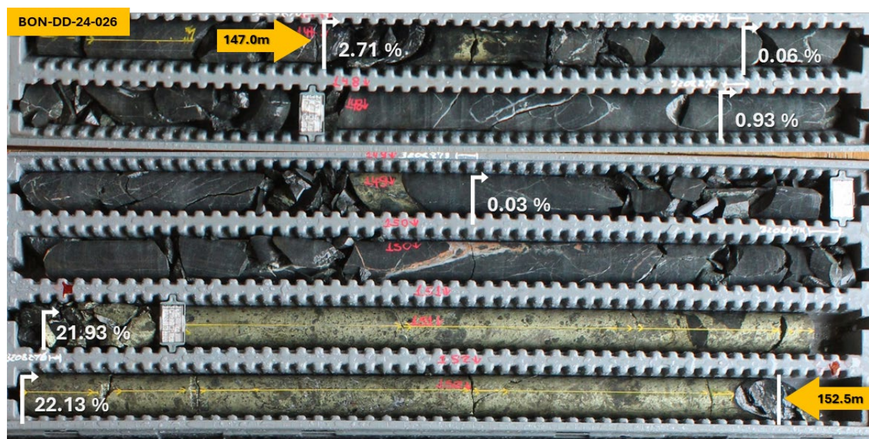
Figure 1 – Nelore Prospect – core photo from drill-hole BON-DD-24-026 Stringer, semi-massive and massive sulphides – chalcopryite (brassy yellow) > pyrrhotite (brown-bronze colour) > pyrite. Assays returned 5.5m at 8.38% Cu and 0.18ppm Au from 147.0m.
