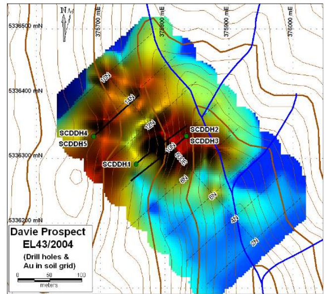
Figure 5: Drill hole location plan with anomalous Au in soil
