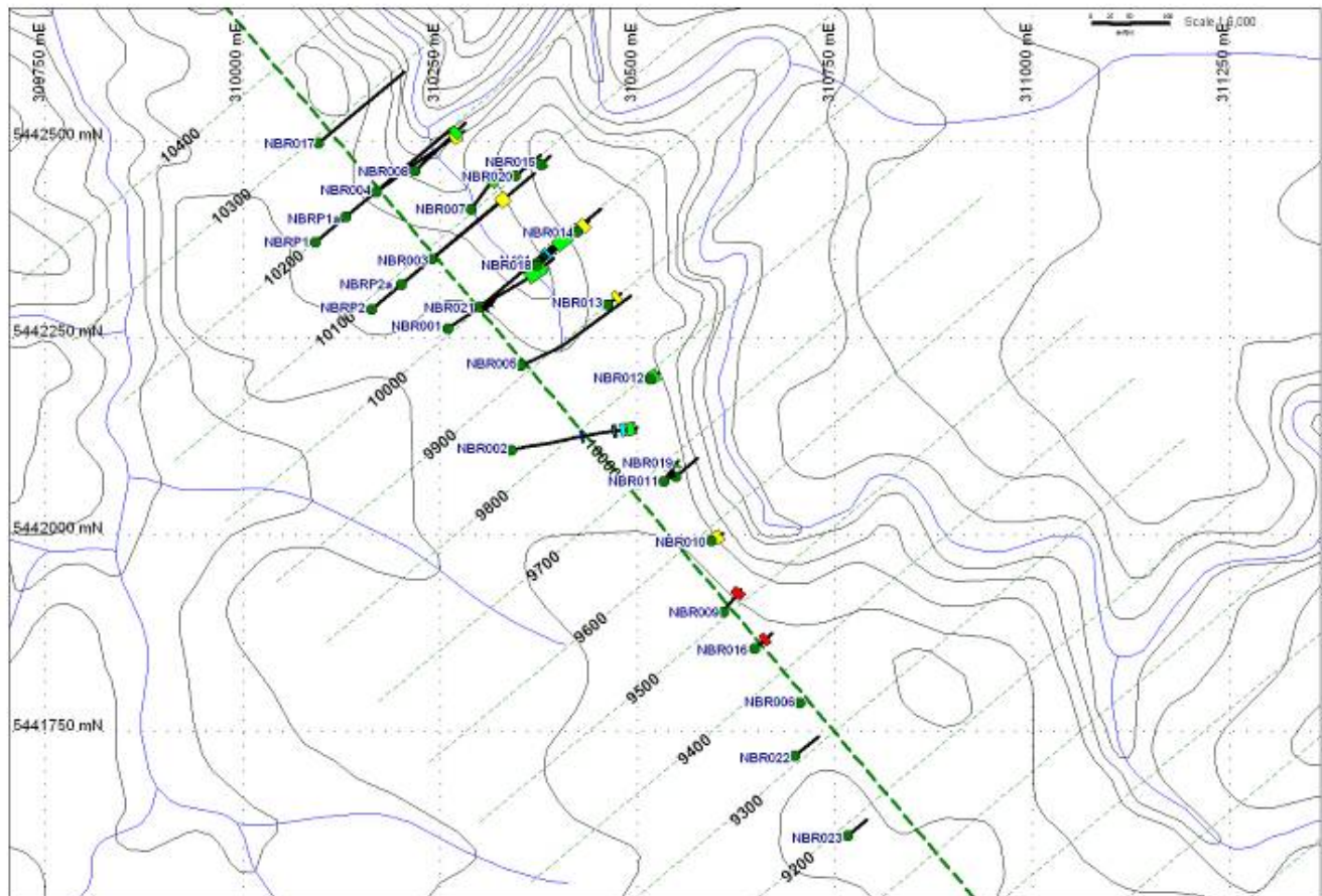
Figure 3: Drillhole location plan - Nelson Bay River Magnetite Project
