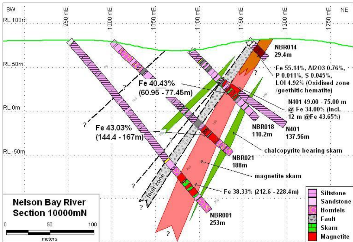
Figure 2: Ore body cross sectional view with mineralisation types and grades
