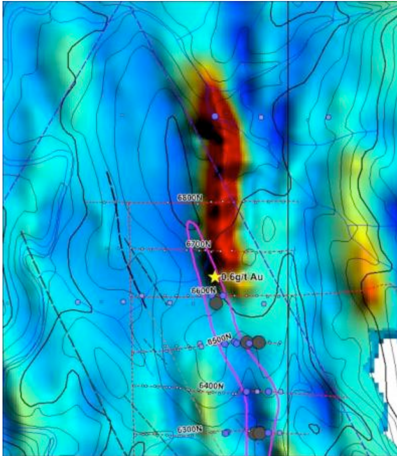
Figure 2: Zn in soils thematic over gridded 1978 chargeability, also showing mafic volcanic (purple), structure (black) and magnetic lineaments (blue)
