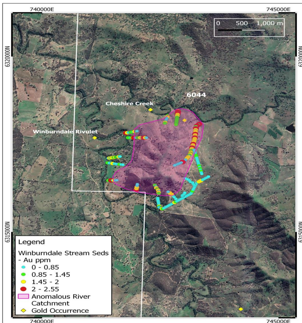
Figure 2. Open File soil and stream-sediment geochemistry (Nickel Mines Ltd., 1972) collected within Shree's EL9017 (formerly ELA6044). An anomalous river catchment area has been outlined.
