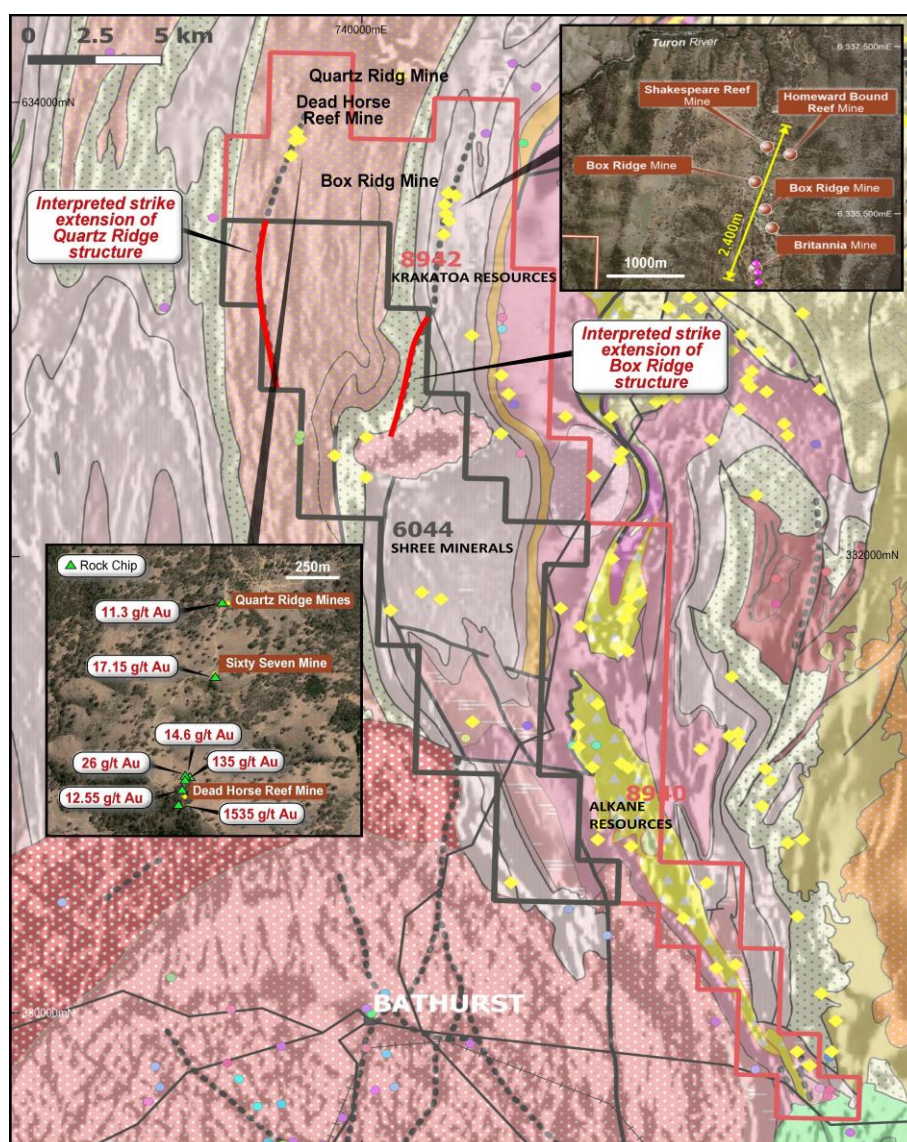
Figure 1. Composite image of the Tuondale Project EL9017 (formerly ELA6044) showing the geology and aeromagnetic structure. Historic gold workings (yellow diamonds) show a north-south trend at the Quartz Ridge and Box Ridge prospects.
