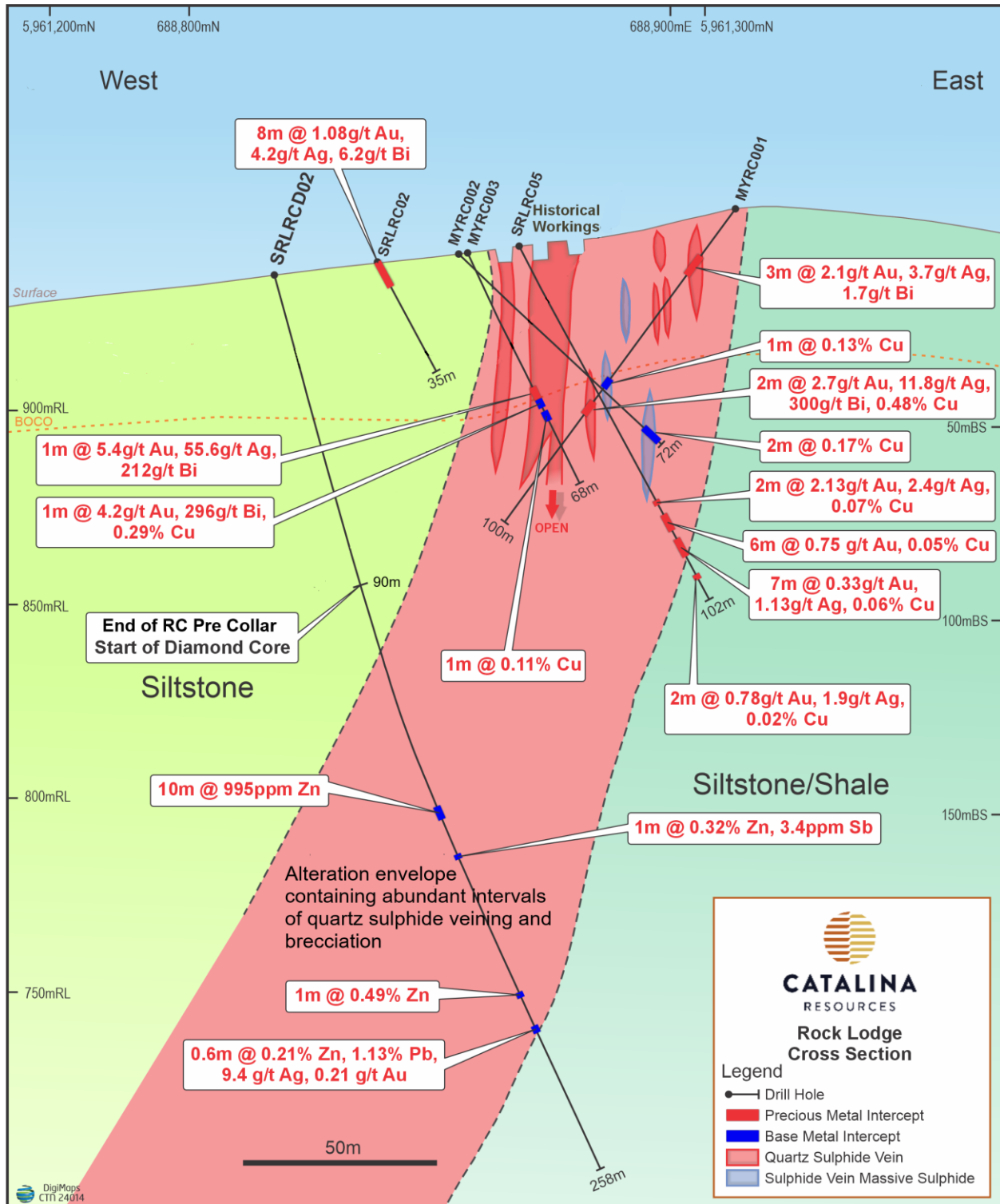
Figure 2: Cross section showing Catalina Resources diamond hole SRLRCD002 testing under previous shallow drilling.
