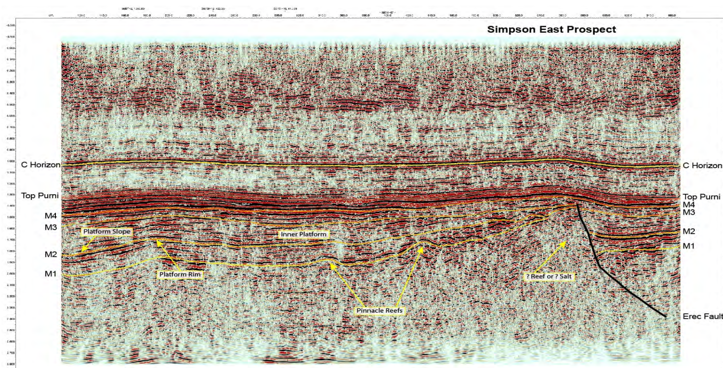
Figures 2 and 3 : Devonian carbonate platform with carbonate mounds developed at the base of the section.
