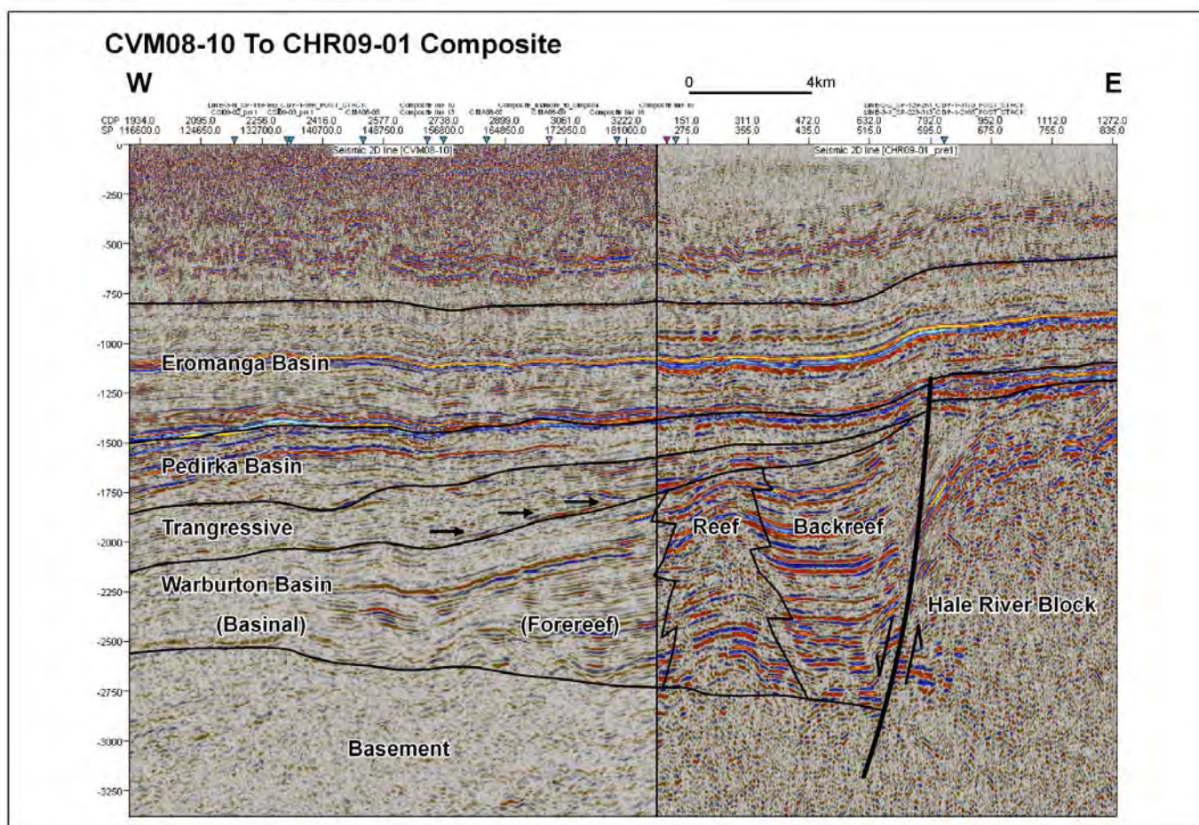
Figure 8: Pellinor Barrier Reef Complex on the margin of the Hale River High (1,500m + vertical expression)
