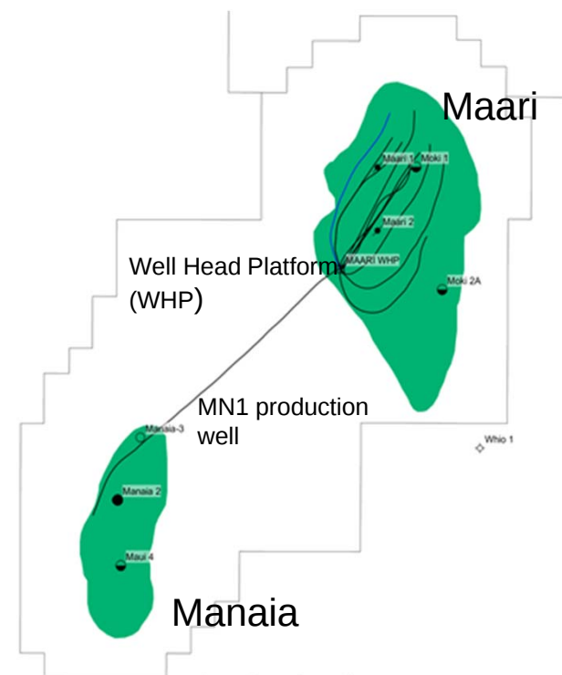
PMP 38160 - Maari and Manaia fields
