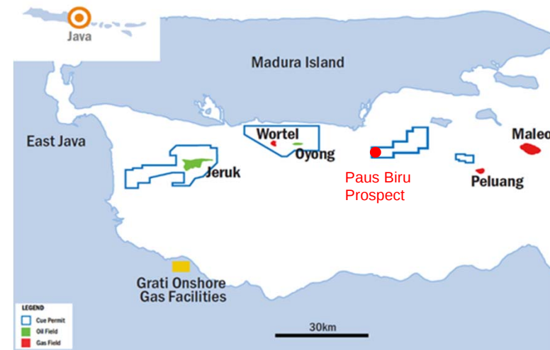
Paus Biru prospect location
