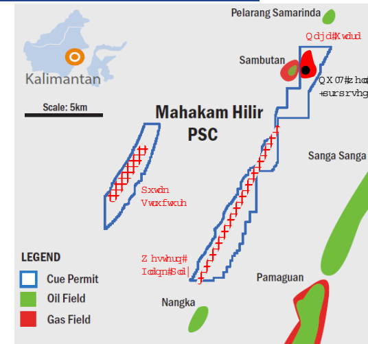
Mahakam Hilir PSC Location
