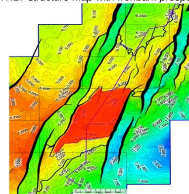
TR17 structure map with Ironbark prospect
